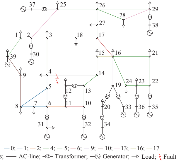
Fig. 5. Topology category of each N-1 outage.
