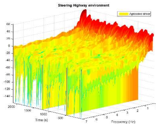
Figure 7. Spectral analysis of the steering wheel movement in highway environment. Signal power (db) is represented in the vertical axis, frequency (Hz) and time representing the moment where the spectral analysis is calculated, are represented in horizontal axis.
