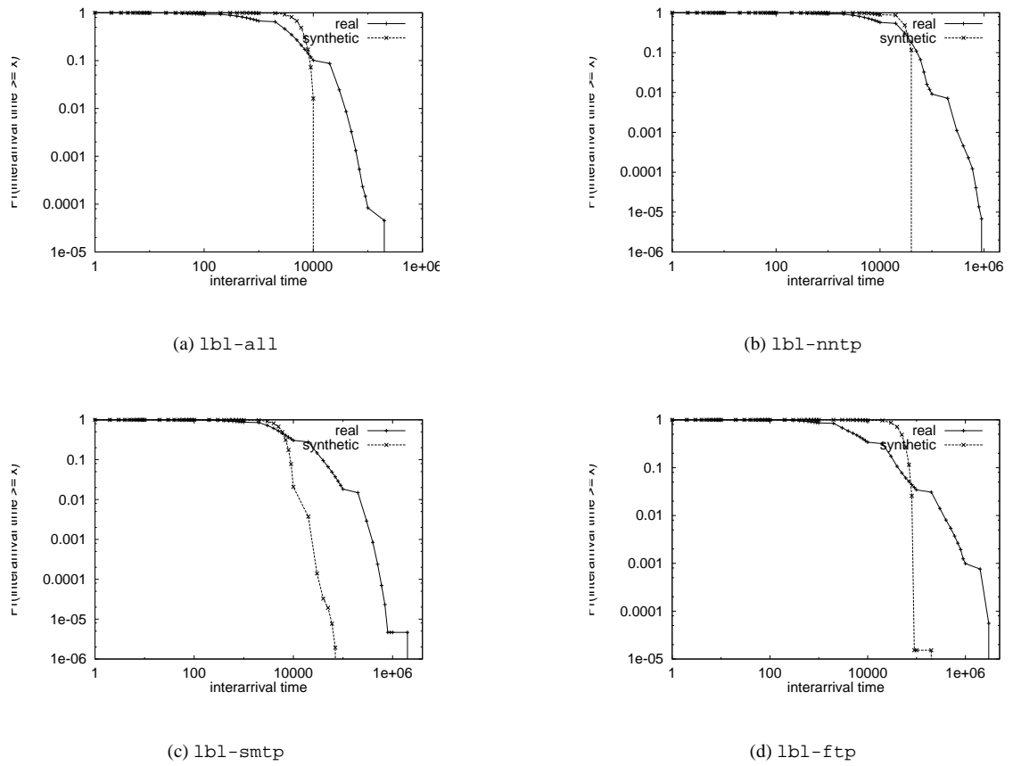
Figure 9: Interarrival time distribution for lbl network traces
