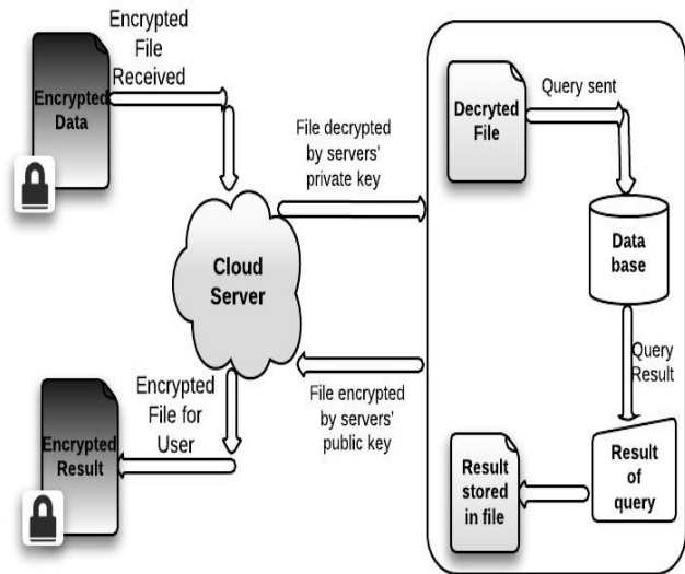
Fig 6: Data Processing view of Server
