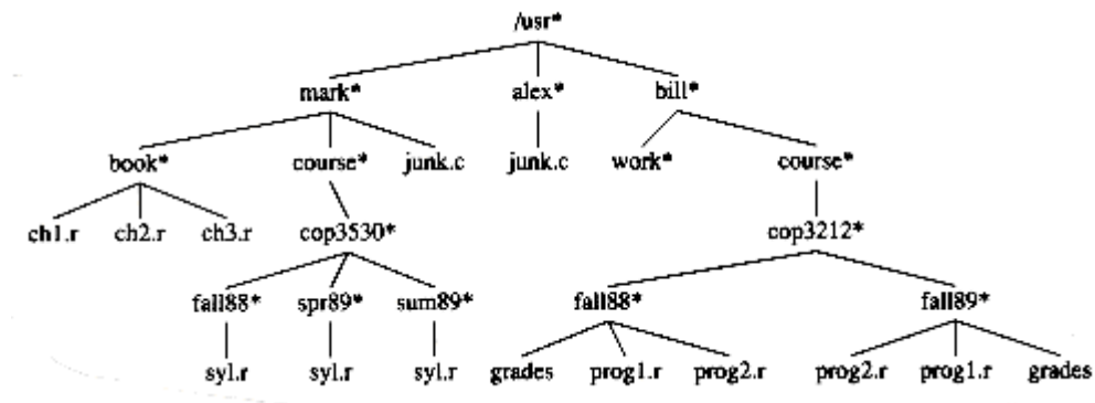
Figure 4.5 Unix directory
