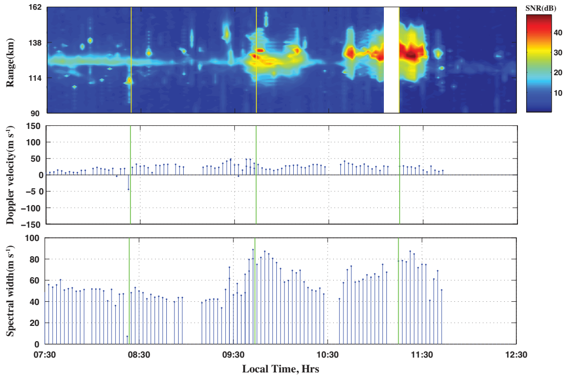
Fig. 3. Range-Time-Intensity map (top panel), Doppler Velocity (middle panel), and spectral width plots (lower panel) obtained from the Chung-Li 52 MHz radar observations on 22 July 2009.
