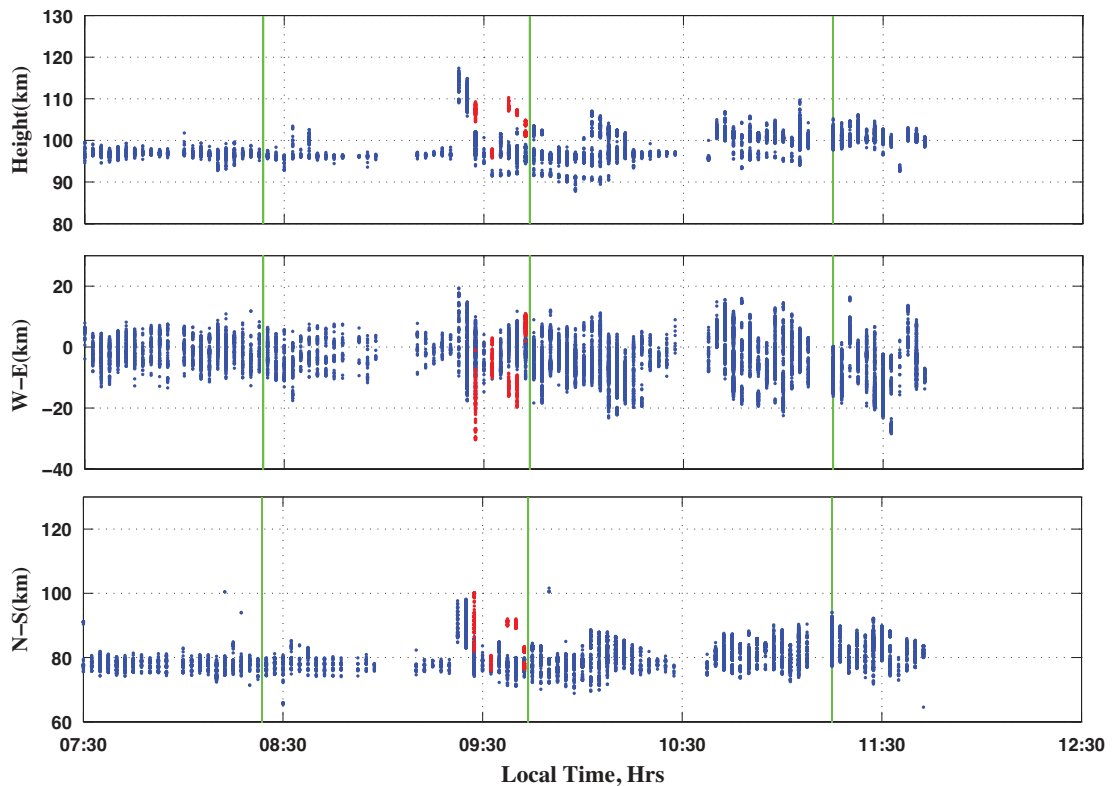
Fig. 4. Time sequences of the interferometer-resolved spatial distributions of Es echoes projected on the vertical (top panel) and horizontal (mid and bottom panels) planes. Note that the presence of short-lived additional layer is shown with red color lines.
