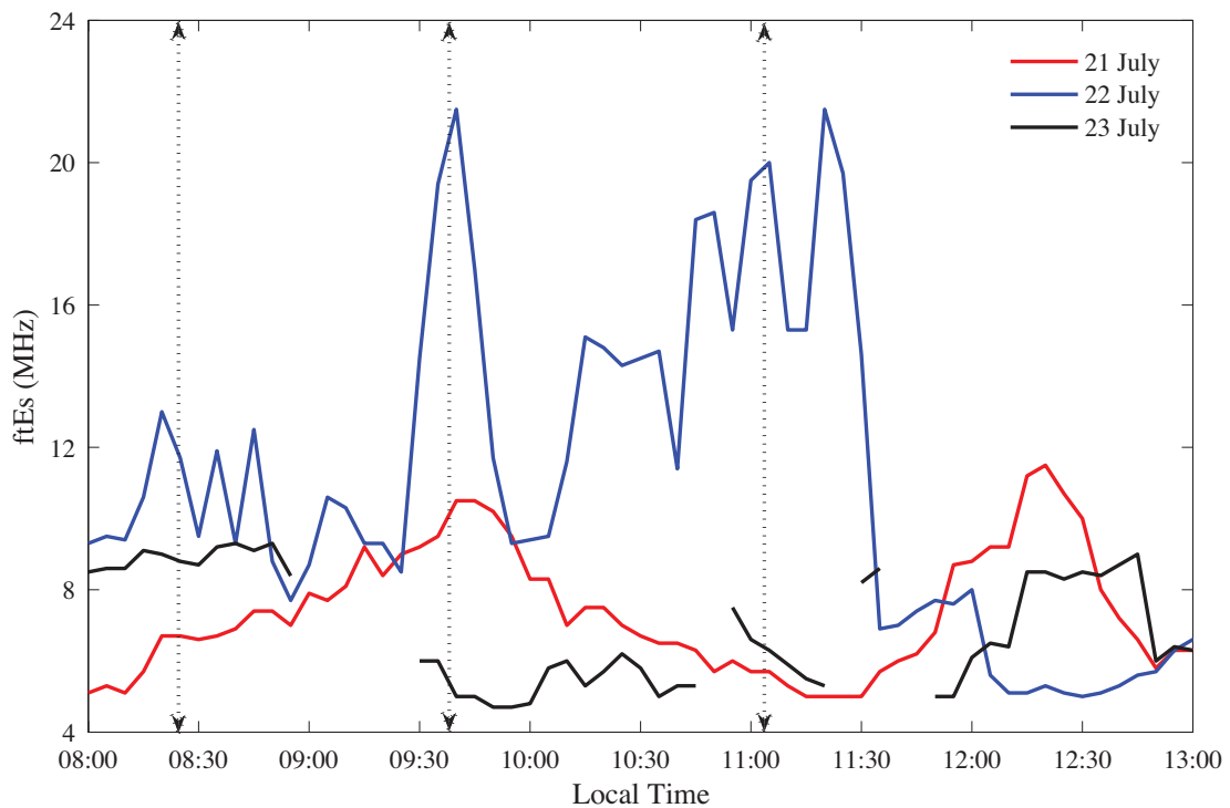
Fig. 6. Ionosonde observations of ftEs from Chung-Li during 21, 22 and 23 July 2009. Note that the initial, peak and final phases of solar eclipse over the Chung-Li radar location are shown with vertical arrow lines.
