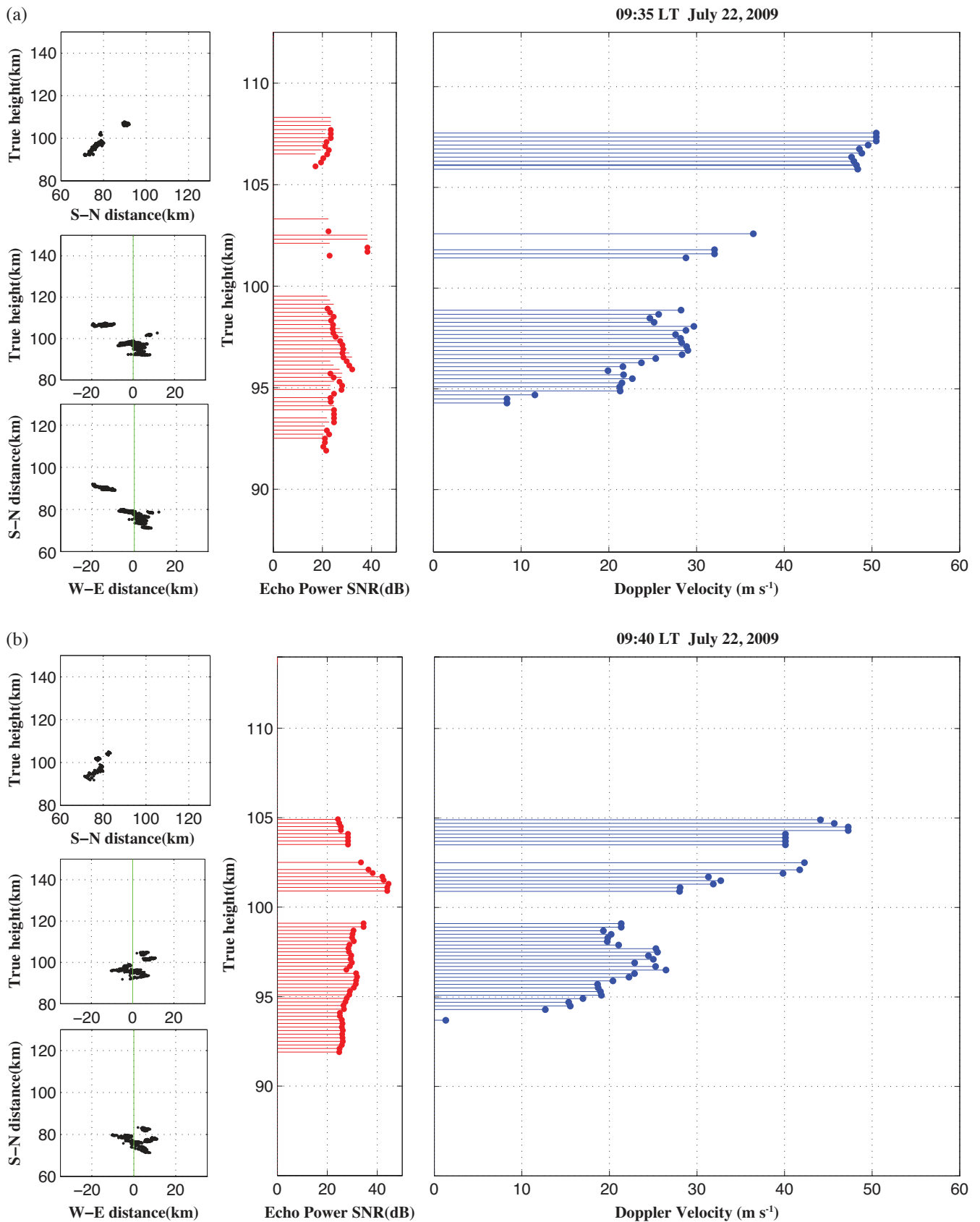
Fig. 8. Interferometer-resolved spatial distributions of Es echoes projected on different planes (both vertical and horizontal), echo power, and Doppler velocities measured using the Chung-Li radar during 0935 LT (a) and 0940 LT (b) on 22 July 2009.
