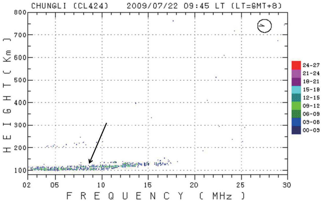
Fig. 5. Typical example of digital ionogram recorded at Chung-Li at 0945 LT on 22 July 2009. Note that the color code represents echo strength in unit dB.
