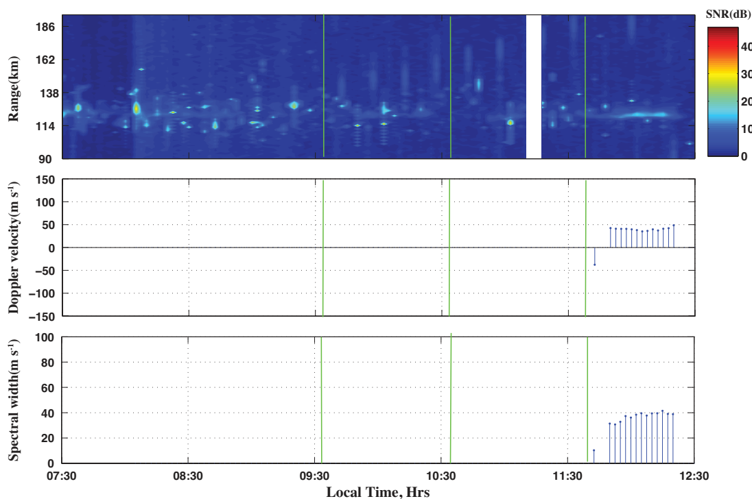
Fig. 2. Range-Time-Intensity map (top panel), Doppler Velocity (middle Panel), and spectral width plots (lower panel) obtained from the Chung-Li 52 MHz radar observations on 21 July 2009.
