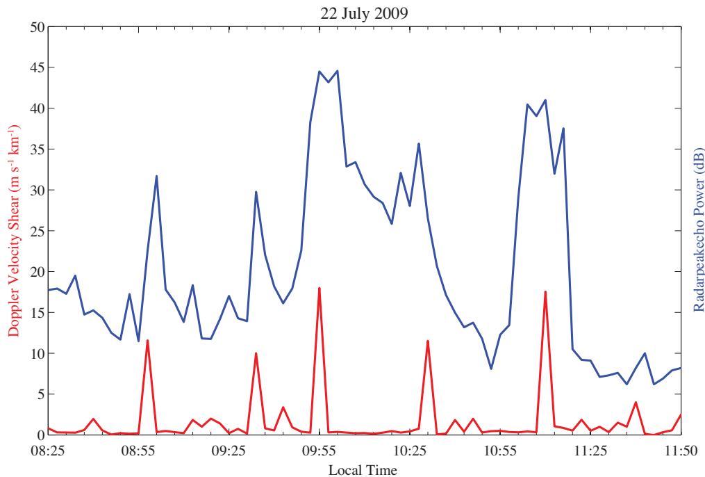
Fig. 9. Comparison between Doppler velocity shear ( \text{m s}^{-1} \text{km}^{-1} ) and radar peak echo power (dB) on 22 July 2009, wherein a one-to-one correspondence between them is clear.
