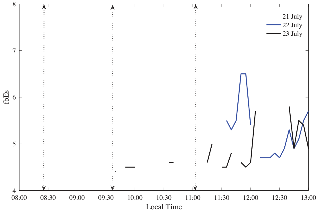
Fig. 7. Ionosonde observations of fbEs from Chung-Li on 21, 22 and 23 July 2009. Note that the initial, peak and final phases of solar eclipse over the Chung-Li radar location are shown with vertical arrow lines.
