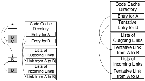
(a) Proactive linking applied to the trace being translated when the branch target is cached.
