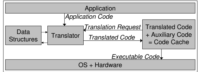
Figure 2. Block diagram of a typical translation-based DBT. The translator is the core of the DBT. It caches its translations and uses data structures to manage the translations.
