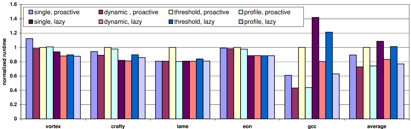
(c) Normalized performance of long-running benchmarks.
