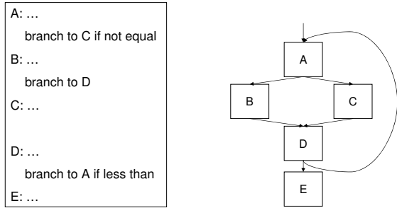
(a) Original code snippet to be translated.
