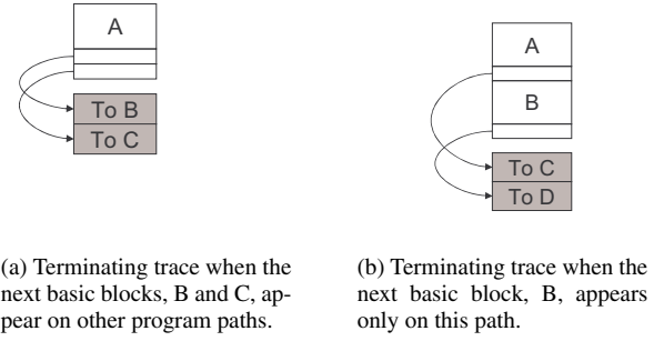
Figure 7. Termination of a trace based on the number of different program paths the next basic block appears in. White areas are parts of the trace while gray areas are exit stubs.
