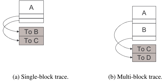
Figure 5. Translation to single-block and multi-block traces. White boxes are parts of the trace, while gray boxes are exit stubs. The gray boxes are labeled with the corresponding CTI targets.
