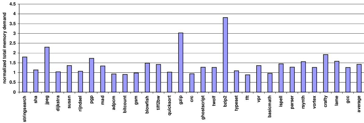
(b) Normalized memory requirements of benchmarks when taken conditional control transfers are elided. Memory efficiency degrades 41% on average.
