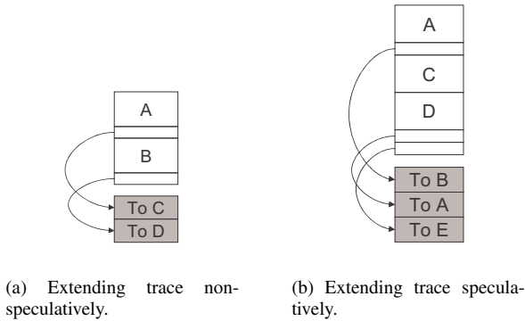
Figure 6. Extending a trace. White areas are parts of the trace while gray areas are exit stubs.
