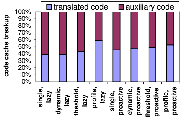
Figure 13. The division between translation code and auxiliary code within the code cache.
