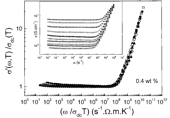
Figure 8. Scaled conductivity [\sigma'(\omega,T)/\sigma_{dc}] vs scaled frequency [\omega/(\sigma_{dc}T)] for p = 0.4 wt % of CNTs in the temperature range 20–110 °C: (□) 20, (●) 30, (△) 40, (▼) 50, (◇) 60, (■) 70, (○) 80, (▲) 90, (▽) 100, and (◆) 110 °C. The inset shows the frequency dependence of the real part \sigma' of the complex conductivity at temperature ranging from 20 to 120 °C for p = 0.4 wt %.
