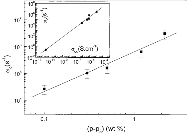
Figure 7. A log–log plot of critical frequency \omega_c vs p - p_c . The solid line is a fit to power law using eq 9. The inset shows the correlation between \omega_c and the dc conductivity \sigma_{dc} at room temperature. The solid line represents the best fitted line for various CNTs content above the percolation threshold. The error bars are within the thickness of the symbols.
