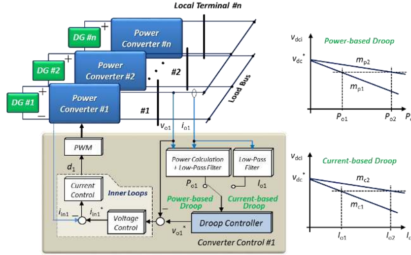
Fig. 3. Control diagram of interface converters based on power- or current-based droop control in DC MGs.
