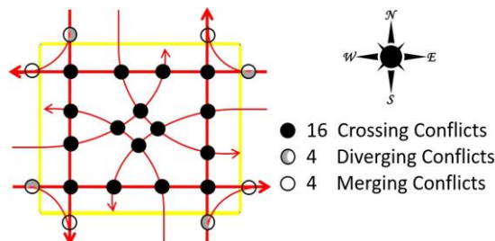
Figure 1: Potential conflicts among all possible crossings in the considered type of intersection.
