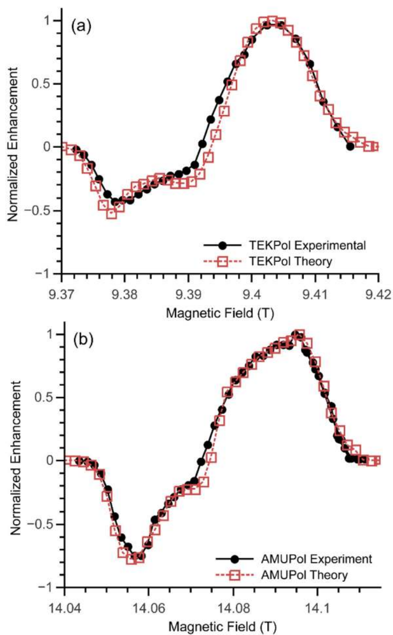
Fig. 5. Experimental (black circles) and simulated (red squares) MAS-DNP field profiles, i.e. the enhancement \epsilon_{\text{on/off}} as a function of the magnetic field while keeping the \mu\omega irradiation frequency constant, for TEKPol (a) and AMUPol (b) at 9.4 T and 14.1 T, respectively.
