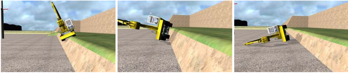
Figure 9: Excavator rollover.
