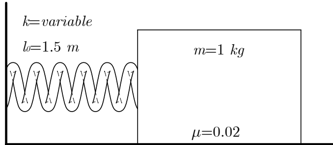
Figure 4: Mass-spring system with Coulomb's friction.
