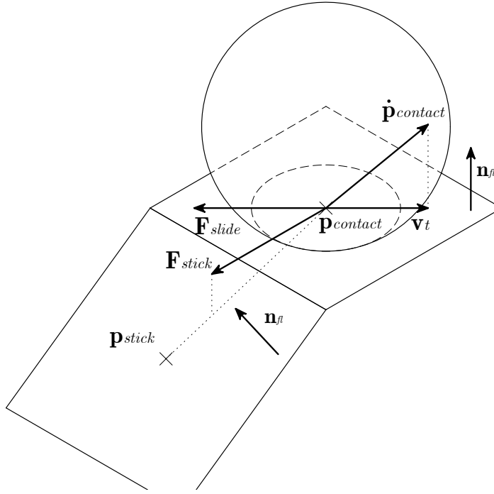
Figure 2: Tangential contact between sphere and plane.
