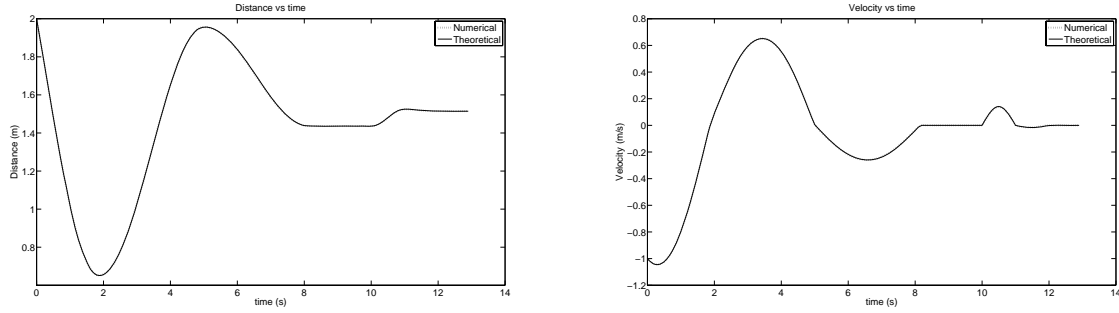
Figure 5: Response of the system (spring distance and velocity): theoretical vs. numerical.
