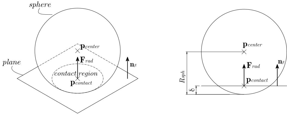
Figure 1: Normal contact between sphere and plane: isometric and front views.
