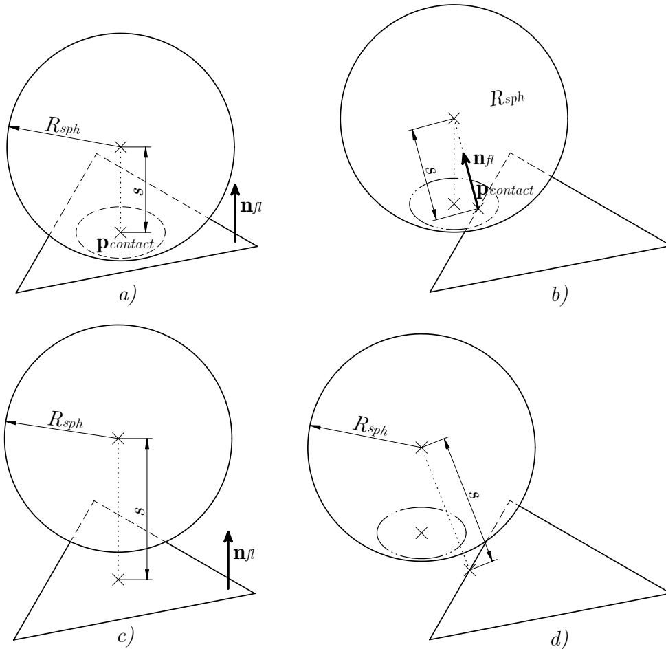
Figure 3: Collision detection between sphere and triangular face.
