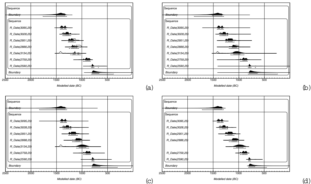
Figure 9 This show a simple sequence under a number of different outlier models: (a) uses the SSimple model as in Christen (2003); (b) uses a t -type outlier model with the offsets distributed as 1007(5) using Outlier_Model("TFixed", T(5), 2, "t") ; (c) uses the General model as defined above with variable scaling; (d) manually removes the obvious outlier and replaces it with an undated event. All outlier models identify the fifth ^{14}\text{C} date as a definite outlier and can be used for outlier detection. However, given that the sample is an outlier, we would expect the modeled output to be similar to that shown in (d) where the date has been excluded: (a) shows that the very prescribed SSimple model pulls the outlier date strongly towards the measurement, even though it is an outlier; (b) which uses a longer-tailed T(5) distribution is more realistic; but (c) gives a better overall model average for this situation since the dated event posteriors are very close to those shown in (d).
