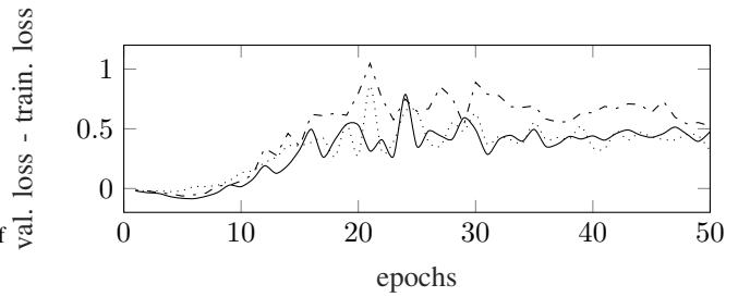
Fig. 2. Difference between both validation and training losses with: \gamma = 1 (continuous line, highest accuracy 74.6%), \gamma = 25 (dotted line, highest accuracy 76.1), \gamma = 100 (the line with the largest dashes, highest accuracy 79.3%). The lower and less spiky the better.
