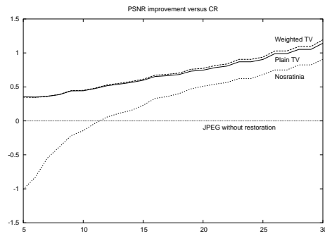
Fig. 1. Improvements of the PSNR versus CR on Lena.
