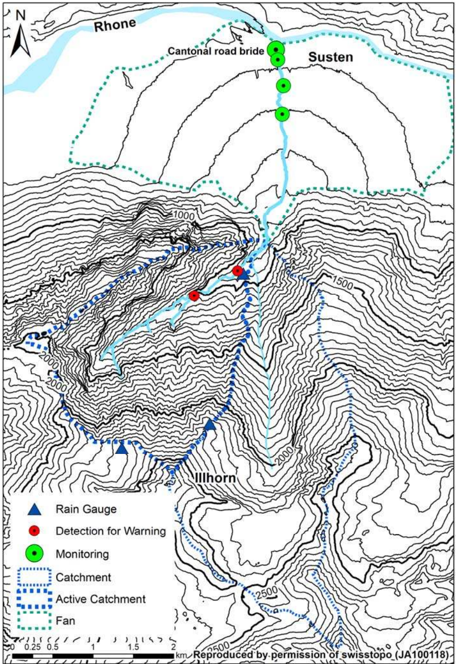
Figure 5: The Illgraben (Switzerland) monitoring site including four stations for monitoring on the fan, two detection stations for the warning in the active catchment and three rain gauges.
