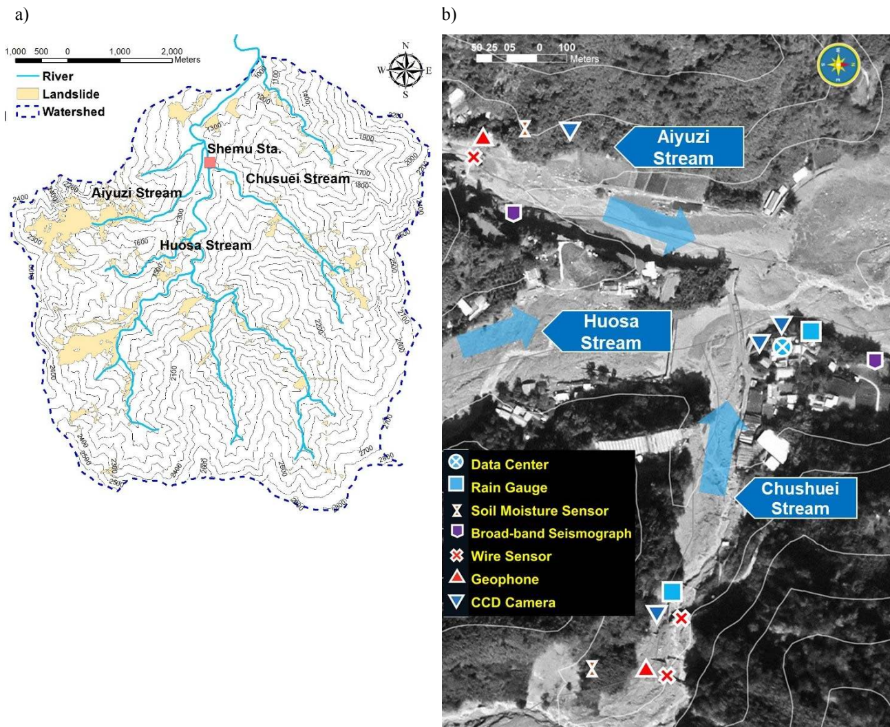
Figure 10: The Shenmu (Taiwan) monitoring site. a) Topographic map and location of the monitoring station at the confluence of the three debris-flow streams (after Lei et al., 2014). b) The layout of sensors installed at the Shenmu monitoring station.
