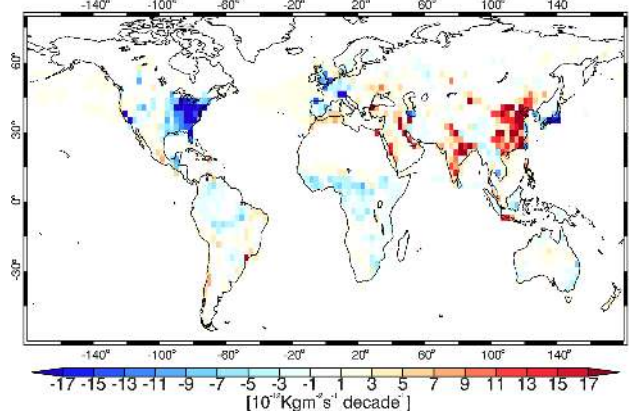
Figure 6. Global distribution of linear trend of the a posteriori surface NO x emissions (in 10^{-12} \text{ kg m}^{-2} \text{ s}^{-1} per decade) for the period 2005–2014. The red (blue) colour indicates positive (negative) trends.
