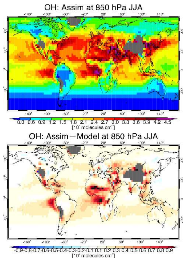
Figure 13. Global distribution of the 10-year mean OH concentration (in 10^6 molecules \text{cm}^{-3} ) in the data assimilation run (top panel) and its difference between the data assimilation run and the model simulation (bottom panel) averaged over June, July, and August over the 2005–2014 period at 850 hPa.
