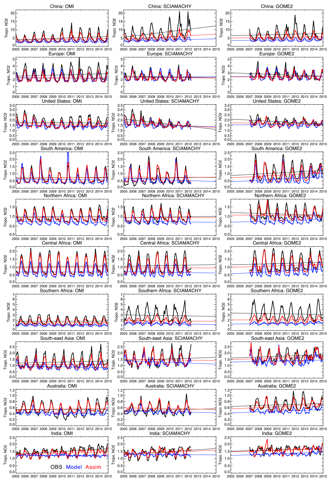
Figure 3. Time series of regional monthly mean tropospheric NO 2 columns (in 10^{15} molec \text{cm}^{-2} ) averaged over China ( 110\text{--}123^\circ E, 30\text{--}40^\circ N), Europe ( 10^\circ W– 30^\circ E, 35\text{--}60^\circ N), the USA ( 70\text{--}125^\circ W, 28\text{--}50^\circ N), South America ( 50\text{--}70^\circ W, 20^\circ S–Equator), northern Africa ( 20^\circ W– 40^\circ E, Equator– 20^\circ N), central Africa ( 10\text{--}40^\circ E, Equator– 20^\circ S), southern Africa ( 25\text{--}34^\circ E, 22\text{--}31^\circ S), South-east Asia ( 96\text{--}105^\circ E, 10\text{--}20^\circ N), Australia ( 113\text{--}155^\circ E, 11\text{--}44^\circ S), and India ( 68\text{--}89^\circ E, 8\text{--}33^\circ N) obtained from the satellite retrievals (black), model simulation (blue), and the data assimilation (red). The model simulation and data assimilation results were obtained at the local overpass time of the retrievals by applying the averaging kernel.
