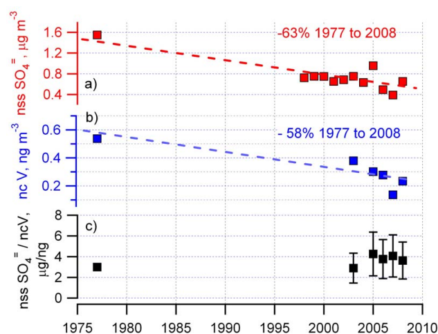
Fig. 2. Concentrations of (a) \text{nss SO}_4^- and (b) \text{ncV} averaged over the haze season (January–April) and (c) the \text{nss SO}_4^-/\text{ncV} ratio. The 1976–1977 data are from Rahn and McCaffrey (1980).
