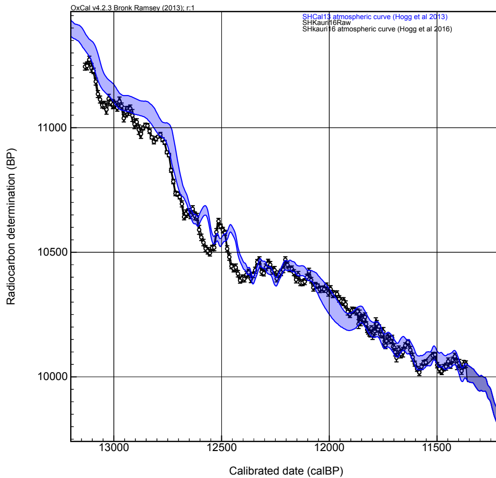
Figure 12. SH (SHkauri16) curve and data points plotted with the SHCal13 curve for the interval 13,200 - 11,200 cal BP. Measured Towai and FIN11 data are appended to IntCal13 RWM data at 11,365 cal BP (see text for more details).
