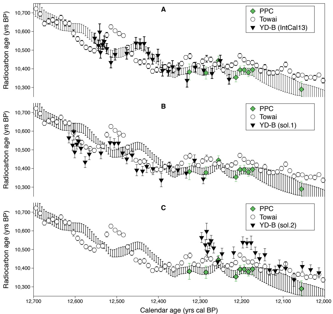
Figure 4. Positioning of ^{14}\text{C} dates from the YD-B tree-ring series. A: As given in IntCal13; B: Curved-matched solution 1; C: Curve-matched solution 2. IntCal13 curve (black 1\sigma error bars) given in all plots.
