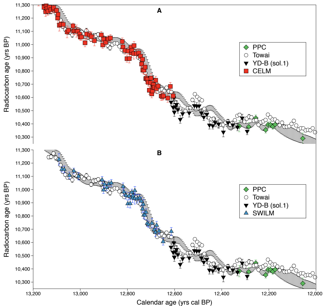
Figure 5. Positioning of ^{14}\text{C} dates from A: the CELM radiocarbon series and B: the SWILM series, compared with the Towai, PPC and YD-B (solution 1) data sets. IntCal13 curve (black 1\sigma error bars) also given.
