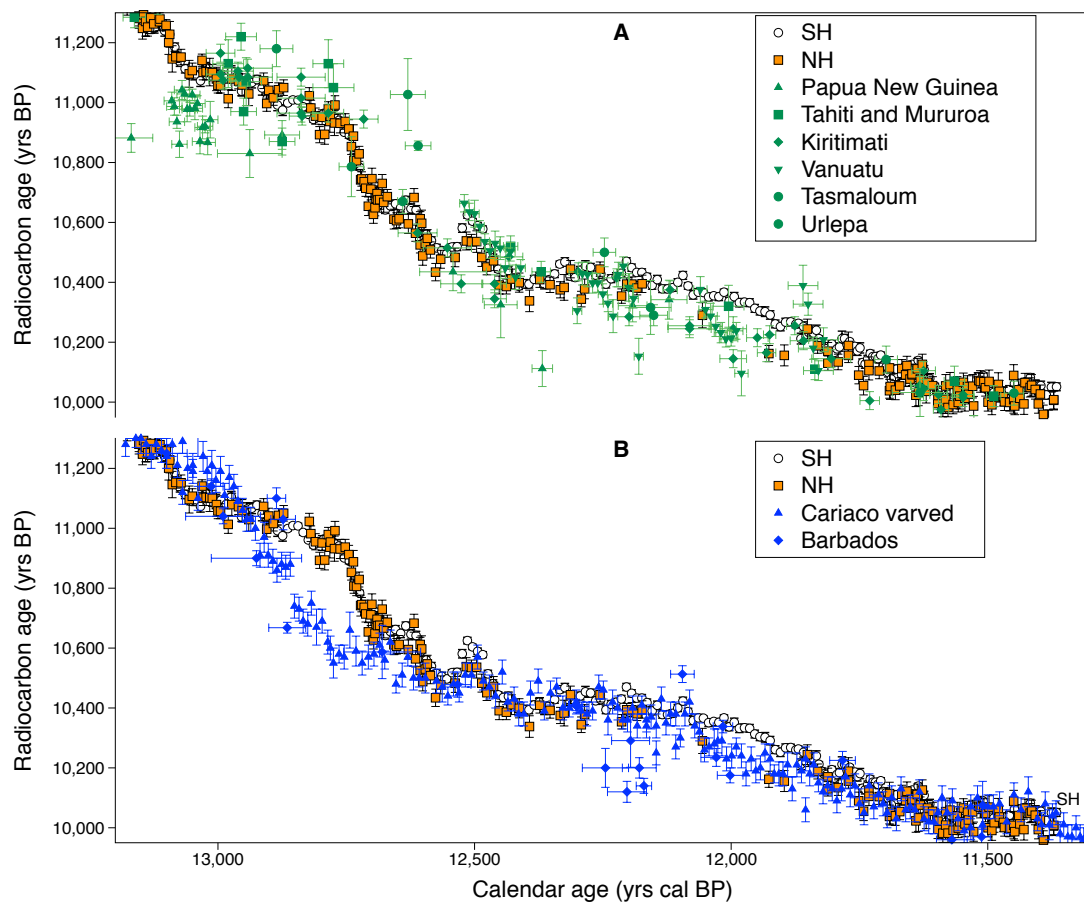
Figure 10. Comparison of marine records with tree-ring ^{14}\text{C} data sets. A: Pacific marine corals (Papua New Guinea; Edwards et al. 1993, Burr et al. 2004, Cutler et al. 2004. Tahiti and Mururoa; Bard et al. 1998, Durand et al. 2013. Kiritimatai; Fairbanks et al. 2005. Vanuatu; Burr et al. 1998. Tasmaloum; Cutler et al. 2004. Urlepa; Cutler et al. 2004) B: North Atlantic marine (Cariaco varved sediments; Hughen et al. 2004, 2006. Barbados corals; Bard et al. 1998 and Fairbanks et al. 2005).
