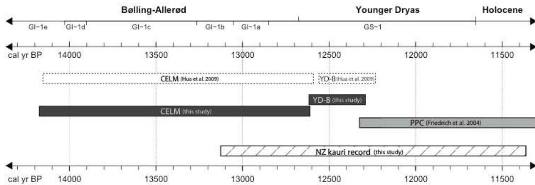
Figure 7. Temporal distribution of Northern and Southern Hemisphere Lateglacial tree-ring chronologies. The SH New Zealand kauri record (cross hatched bar) has been locked to the absolutely dated Preboreal Pine chronology (light grey; PPC; Friedrich et al. 2004) by ^{14}\text{C} and serves as a radiocarbon backbone through the Younger Dryas. The new kauri record enabled accurate curve matching of the Northern Hemispheric floating Central European Lateglacial Master Chronology (black; CELM; Kaiser et al. 2012) and Younger Dryas B (black; YD-B; Hua et al. 2009). The former positions of the CELM and YD-B chronologies (dashed lines; Hua et al. 2009) are revised and adjusted in this work. The starting series of the PPC in this diagram is the Cottbus chronology beginning at 12,325 cal BP: the ‘Zurich’ pine KW30 series is the end (youngest) member of the Hua et al. (2009) YD-B series. In addition to the calendar timescale (cal BP), the diagram also shows the INTIMATE Greenland Isotope event stratigraphy (on the GICC05 time scale in cal BP; Blockley et al. 2012, Rasmussen et al. 2014) and European climate stratigraphy, including the Lateglacial Interstadial (the Bølling/Allerød); the onset of the YD is as given in Rach et al. (2014).
