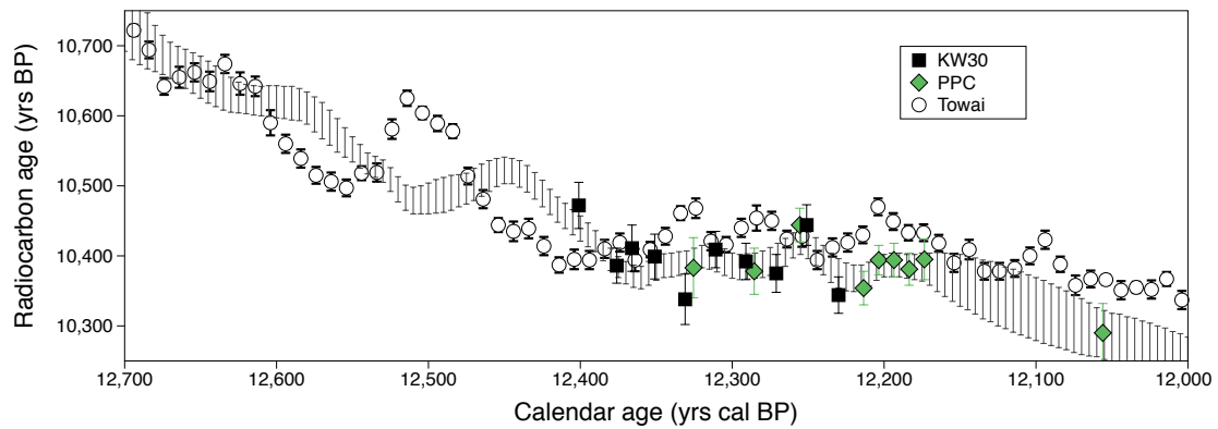
Figure 3. Positioning of YD-B KW30 measurements as included in IntCal13 (data as tabulated in the IntCal13 database - HD atmospheric, Set 5 Division 2). IntCal13 curve (black 1\sigma error bars) is also given.
