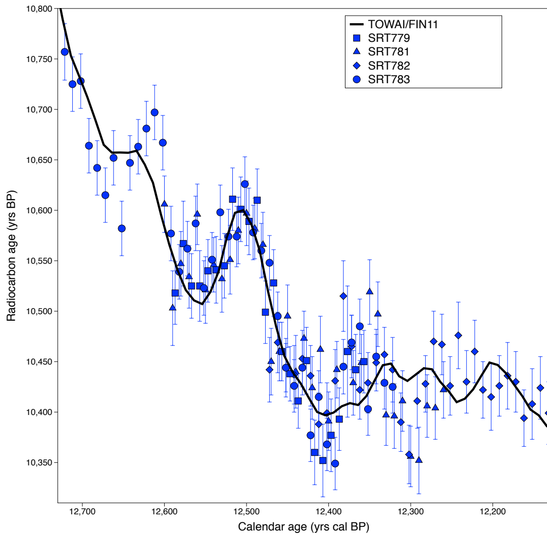
Figure 8. Tasmanian huon data sets (Hua et al. 2009) plotted with Towai/FIN11 5-pt moving average.
