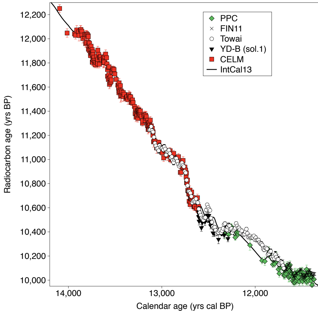
Figure 6. The complete SH Towai and FIN11 14 C time series plotted with the NH CELM, YD-B and PPC data sets. IntCal13 curve shown as a black line.
