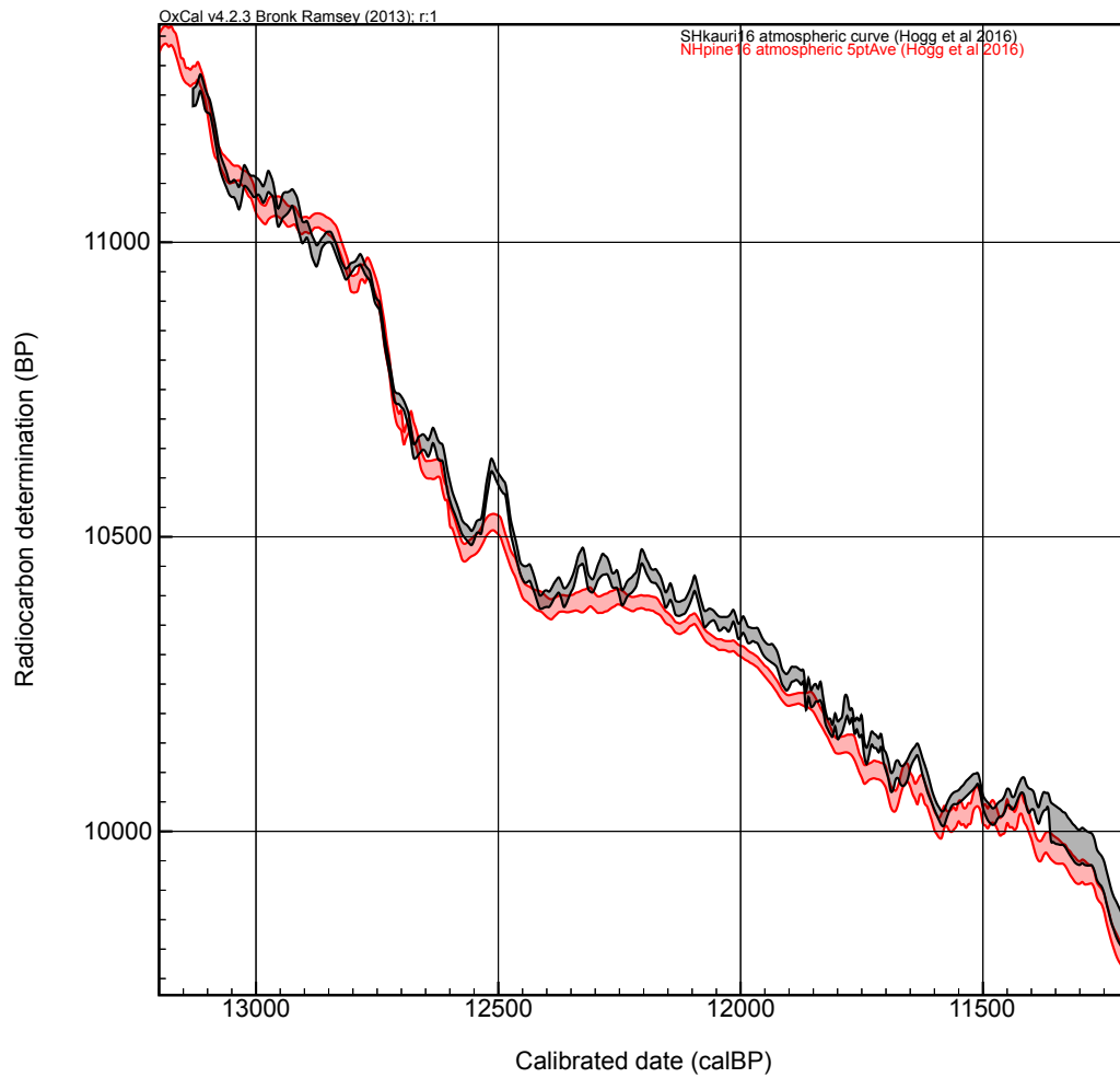
Figure 11. SH (SHkauri16, black) and NH (NHpine16, red) comparison curves for the interval 13,200 - 11,200 cal BP (see text for more details).
