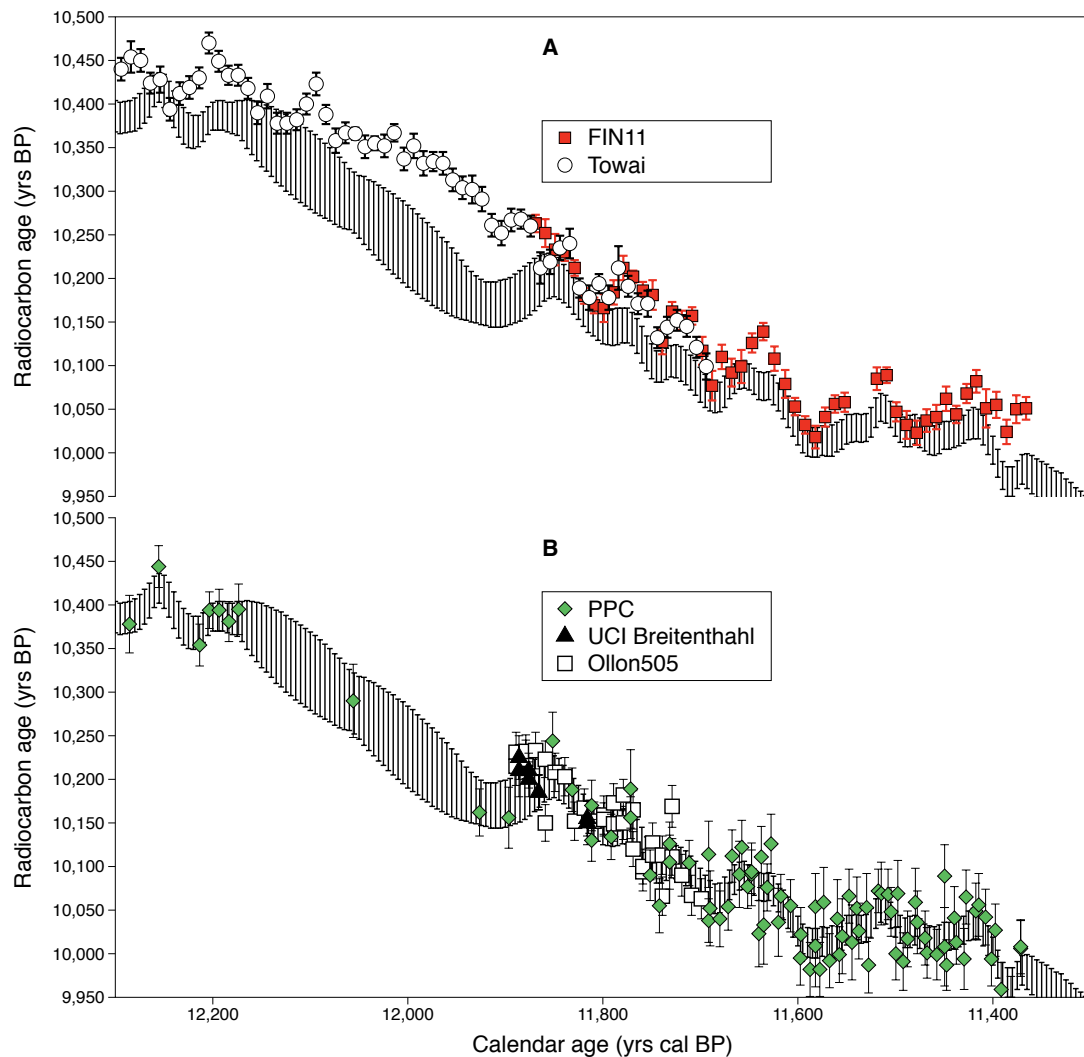
Figure 2. A: Floating SH Towai and FIN11 datasets. 2B: NH datasets. (i) Known calendar-age: Preboreal pine chronology (PPC) and Breitenhahl (UCI); (ii) Floating: Ollon505 (new Wk and HD data; Hogg et al. 2013a). IntCal13 curve (black 1\sigma error bars) given in both plots.
