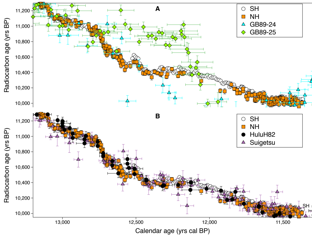
Figure 9. Comparison of YD terrestrial records with tree-ring ^{14}\text{C} data sets. A: GB89-24 (Beck et al. 2001) and GB89-25 (Hoffmann et al. 2010) speleothems and B: HuluH82 speleothem (Southon et al. 2012) and Lake Suigetsu macrofossils (Bronk Ramsey et al. 2012).
