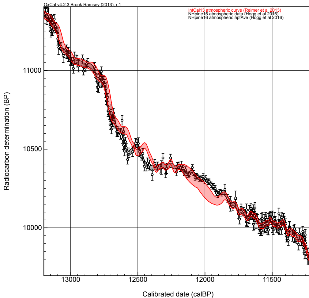
Figure 13. NH (NHpine16) curve and data points plotted with the IntCal13 curve for the interval 13,200 - 11,200 cal BP. A 5-point moving average has been applied to the revised decadal NH data points, from 14,120 - 11,420 cal BP. IntCal13 RWM data is appended at 11,415 cal BP (see text for more details).
