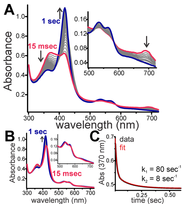
Figure 2. Reaction of OleT JE :eicosanoic acid with H 2 O 2 . A 20 \mu M E-S complex prepared with a perdeuterated substrate (A) or protiated substrate (B) was rapidly mixed with 5 mM H 2 O 2 at 5 °C. (C) Single turnover time course for the decay of Compound I in reactions with perdeuterated eicosanoic acid. A two summed exponential fit (red) is shown superimposed on the data.
