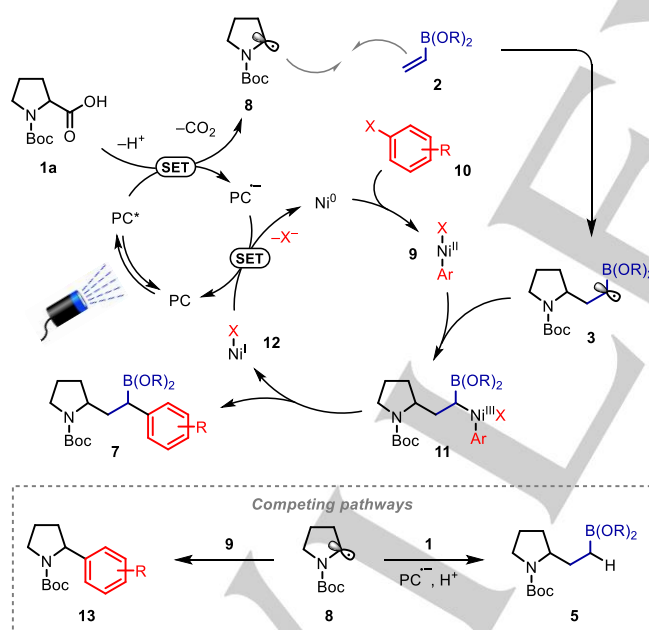
Scheme 2. Proposed mechanism.
