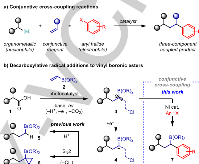
Scheme 1. Conjunctive cross-coupling reactions and decarboxylative radical additions to vinyl boronic esters.
