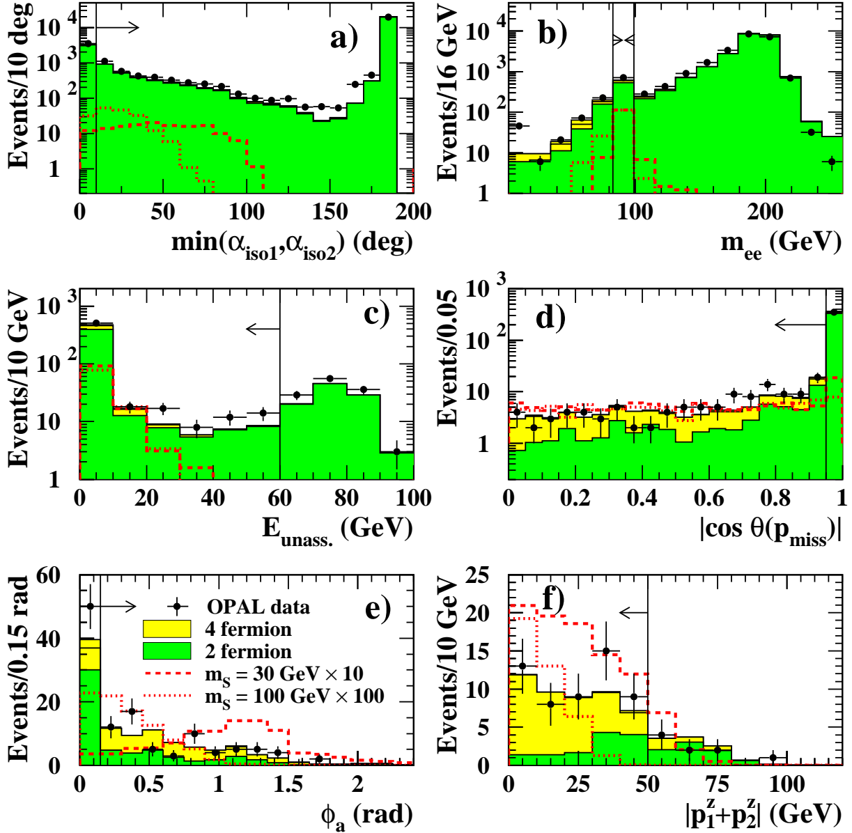
Figure 5: Cut variables for Z^0 \rightarrow e^+e^- at \sqrt{s} = 183\text{-}209 GeV. The OPAL data are indicated by dots with error bars (statistical error), the four-fermion background by the light grey histograms and the two-fermion background by the medium grey histograms. The signal distributions from a 30 GeV S^0 are plotted as dashed lines and those from a 100 GeV S^0 as dotted lines, respectively. The signal histograms are normalised to 10 and 100 times of the Standard Model Higgs-strahlung cross section, respectively, and show the decays S^0 \rightarrow gg . Each variable is shown with the cuts applied before the cut on this variable is done, respecting the order of cuts in Table 4. The arrows indicate the accepted regions.
