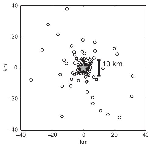
Figure 1 | Combined aftershocks of M = 3–4 mainshocks. To create a composite aftershock data set, we move all of the mainshocks to the origin in space and time and move their aftershocks with them. Data here are for the first 30 minutes of aftershocks of M = 3–4 mainshocks. The grey star gives the locations of the mainshocks, at the origin.
