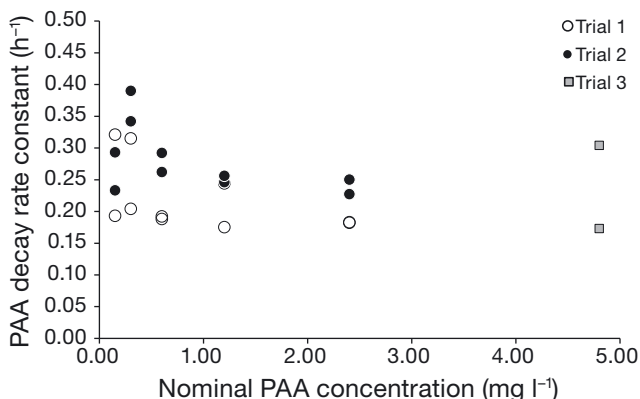
Fig. 5. Calculated decay rate constants PAA derived from trials with addition of PAA to tanks with 300 l seawater at 15^\circ\text{C} in initial concentrations of 0.15 , 0.30 , 0.60 , 1.20 and 2.4 \text{ mg l}^{-1} PAA ( n = 20 ). Each symbol represents a calculated PAA decay rate constant from an individual tank trial. Trial 1 included 25 \text{ kg m}^{-3} salmon post-smolts exposed for 5 min, and trial 2 included 10 \text{ kg} post-smolts exposed to PAA for 30 min before transfer. The grey squares represent a subsequent trial where 4.8 \text{ mg l}^{-1} PAA was added to 2 tanks with 500 l seawater ( 15^\circ\text{C} ) in which 15 \text{ kg m}^{-3} post-smolts were exposed to PAA for 30 min ( n = 2 )
