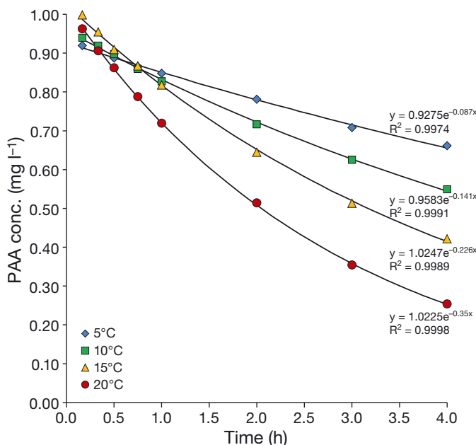
Fig. 1. Peracetic acid (PAA) decay in full-strength seawater at 4 different temperatures. Symbols reflect average PAA concentration ( n = 3 ) with the respective first-order exponential regression lines (Eq. 2)
