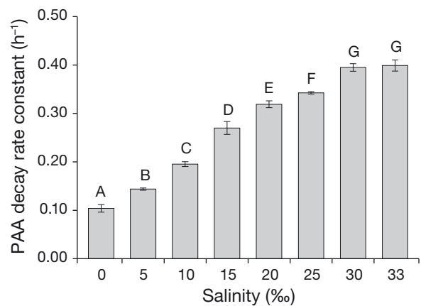
Fig. 3. Calculated first-order PAA degradation rate constants (mean \pm SD; n = 3 ) according to salinity, based on batch experiments performed at 20^\circ\text{C} with nominal PAA concentration at 1 \text{ mg l}^{-1} . All data are based on true triplicate experiments. Different letters denote significant difference ( p < 0.05 )
