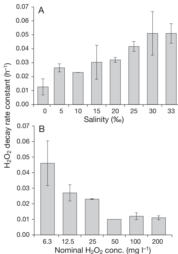
Fig. 6. (A) Calculated decay rate constants of \text{H}_2\text{O}_2 (mean \pm SD) derived from beaker experiments at 20^\circ\text{C} . Divosan Forte was added to water samples with different salinities at an initial concentration ( C_0 ) of 1 \text{ mg l}^{-1} PAA which corresponded to a C_0 of 1.6 \text{ mg H}_2\text{O}_2 \text{ l}^{-1} . (B) Decay rate constants of \text{H}_2\text{O}_2 (mean \pm SD) derived from beaker experiments at 22^\circ\text{C} with different initial \text{H}_2\text{O}_2 concentration added to full-strength seawater. Values are based on duplicate experiments, except C_0 = 50 \text{ mg H}_2\text{O}_2 \text{ l}^{-1} where an outlier is removed
