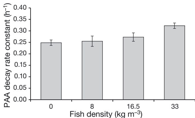
Fig. 4. Calculated decay rate constants of PAA (mean \pm SD) when added to 300 l tanks ( n = 20 ) with full-strength seawater and different biomasses (fish densities). Each bar represents a calculated PAA decay rate constant from an individual tank trial. The nominal concentration of PAA was 1.0 \text{ mg l}^{-1} , water temperature was 15.2\text{--}15.8^\circ\text{C}
