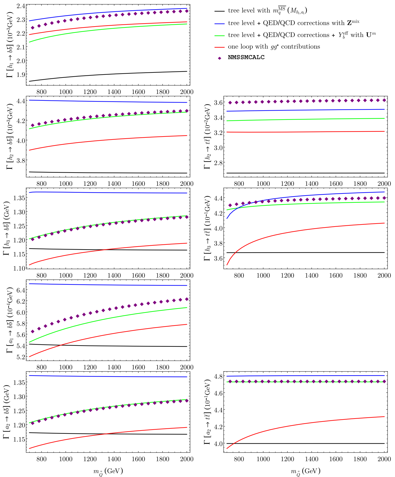
Fig. 6 Comparison with NMSMICALC of the decay widths of the Higgs states into b\bar{b} and t\bar{t} . The input parameters are provided in Table 1. The black lines are pure tree-level results; for the blue lines, QCD and QED corrections are included and the Higgs states are transformed to the loop-corrected eigenstates using \mathbf{Z}^{\text{mix}} ; the green curves
