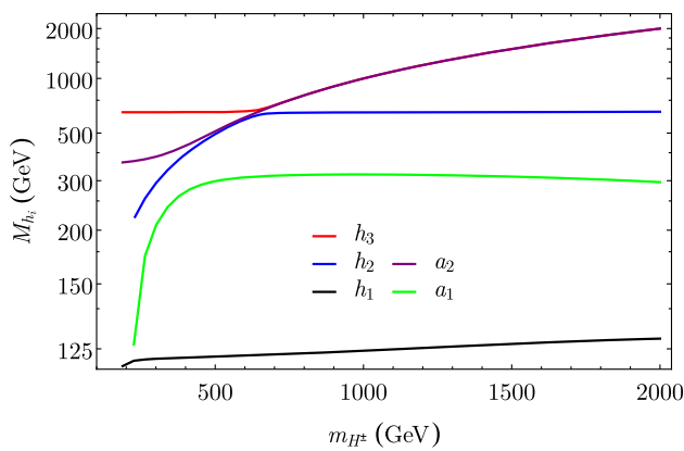
Fig. 7 Higgs masses in the scenario of Fig. 8
