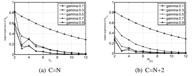
Fig. 15. Largest eigenvalue vs N_{(C)} for L-ZC, various \gamma values, numerical results
