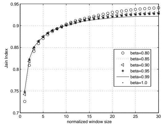
Fig. 5. Jain's index vs normalised window size, m , L-MAC with different values of \beta , C = 16 , 16 stations. Ns-2 simulations
