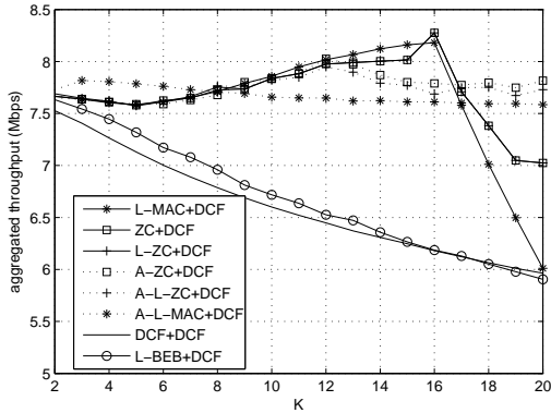
Fig. 13. Network throughput for a network N = 2K stations of mixed MACs. K of the stations use DCF, and K use another MAC. C = 16 for MACs with fixed schedule length. Ns-2 simulations
