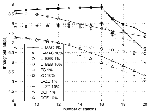
Fig. 11. Network throughput vs number of stations with errors, comparison between DCF and MACs with fixed schedule length, ns-2 simulations, C = 16
