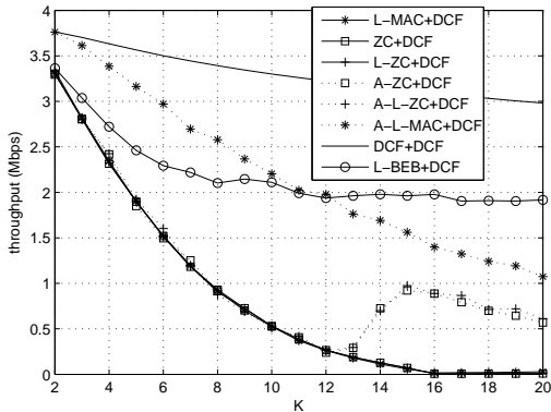
Fig. 14. Throughput for DCF stations in network of N = 2K stations of mixed MACs. K of the stations use DCF, and K use another MAC. C = 16 for MACs with fixed schedule length. Ns-2 simulations
