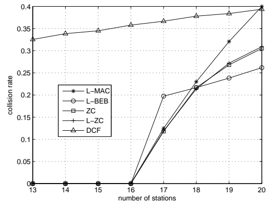
Fig. 9. Collision rate vs. number of stations, comparison of MACs, ns-2 simulations, C = 16
