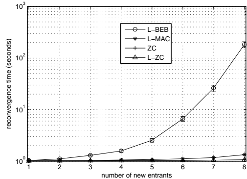
Fig. 12. Reconvergence time when N = 8 stations are in the network and a variable number of stations are added, resulting in N = 9 to N = 16 . ns-2 simulations, C = 16
