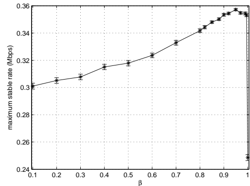
Fig. 6. Achievable stable symmetric rate for different values of \beta . L-MAC, C = 16 , N = 20 stations, ns-2 simulations
