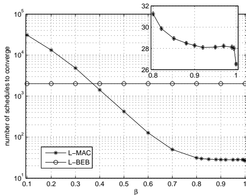
Fig. 4. L-MAC's convergence time for a range of learning strengths, \beta , and L-BEB on log scale. C = 16 , N = 16 stations. The inset graph shows the detail for \beta \in (0.8, 1) on a linear scale. Ns-2 simulations
