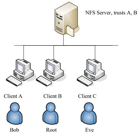
Fig. 7. NFS trust model when using the AUTH_SYS authentication flavor (adopted from [Callaghan 2000]). The NFS server trusts client hosts A and B. Access control is enforced by inspecting the source IP address of RPC requests. User Bob can legitimately access his files after authenticating to client A. However, a privileged user on client B (Root) can easily assume the credential of Bob without knowledge of his password. Finally, user Eve on client C can spoof the IP address of client A. Thus, RPC requests from C appear to come from A, and client C is trusted, though it is not in the server’s access list!
