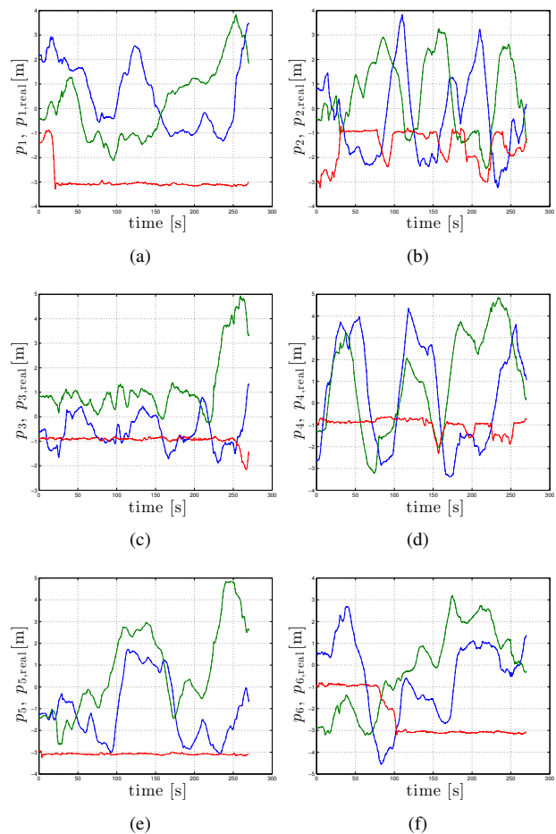
Fig. 11. Figs. (a–f): behavior of p_i(t) (solid) and p_{i,real} (dashed): these are basically superimposed, showing the accuracy of the quadrotors in tracking the reference trajectory p_i(t) . In the plots the following color code is used: blue/red/green solid/dashed lines correspond to the x/y/z components of p_i(t) and p_{i,real}
