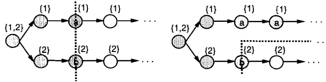
Fig. 4. Maximal configuration for the formula \exists\Diamond(a \wedge b) in two different causal structures. Note that in one case, the maximal configuration is infinite for process 1.
