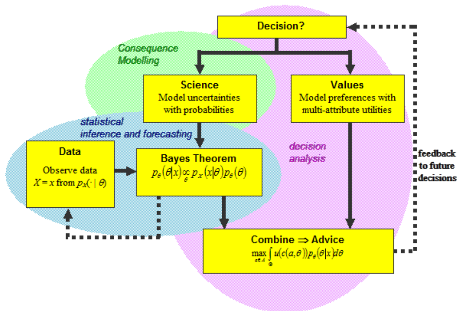
Figure 1: The Bayesian Paradigm (modified from French, 2003) The topmost box represents the issue and problem formulation in which the need for a decision is recognised and the analysis structured to separate the Science of what might happen and what might be done from Value judgements about the potential outcomes. In the obvious notation, p is used for the decision-maker's probabilities, u for her utilities, c(a, \theta) for the consequence of her action a when the state of the world is \theta .
