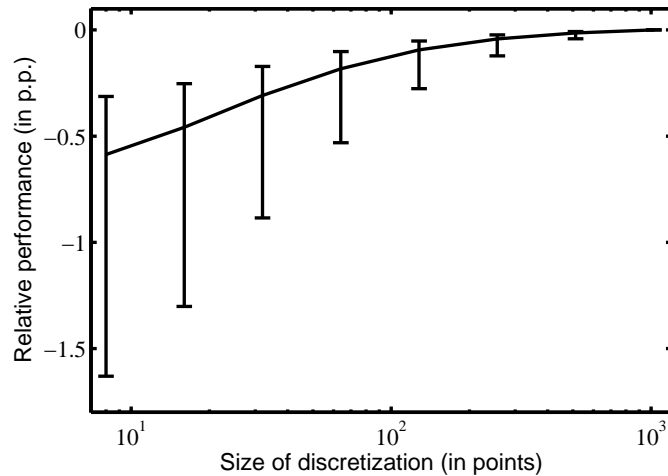
Figure 1: Statistics of convergence of approximate optimal worst-case certainty equivalent when prudence is accounted for using a discretization grid of growing size. The average, 10th, and 90th centile of the performance relative to the performance achieved with a grid of 1000 points is presented for a set of 6000 experiments.
