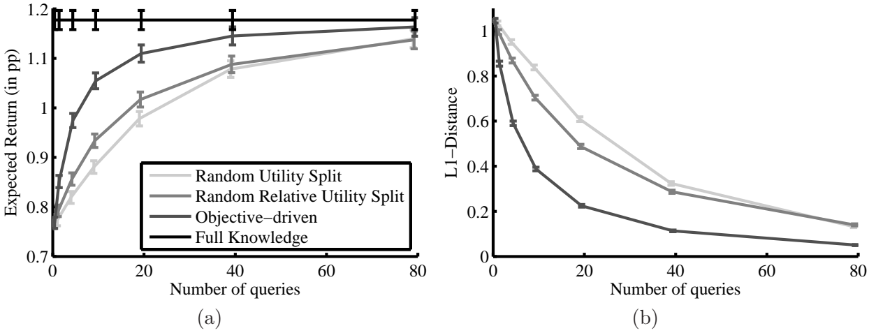
Figure 3: Effect of increasing numbers of questions in a stochastic domination formulation: (a) presents the expected return (in percentage points) and (b) presents the L1-distance between optimal allocation with K queries and the optimal allocation with full knowledge. Shown are averages and standard errors from 1500 simulations.
