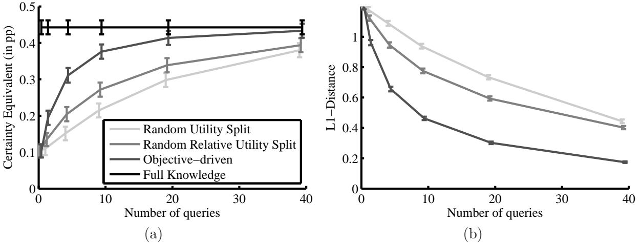
Figure 4: Effect of increasing numbers of questions in a robust certainty equivalent formulation: (a) presents the certainty equivalent (in percentage points) of the optimal portfolio as measured with respect to the true utility function and (b) presents the L1-distance between optimal allocation with K queries and the optimal allocation with full knowledge. Shown are averages and standard errors from 500 simulations.
