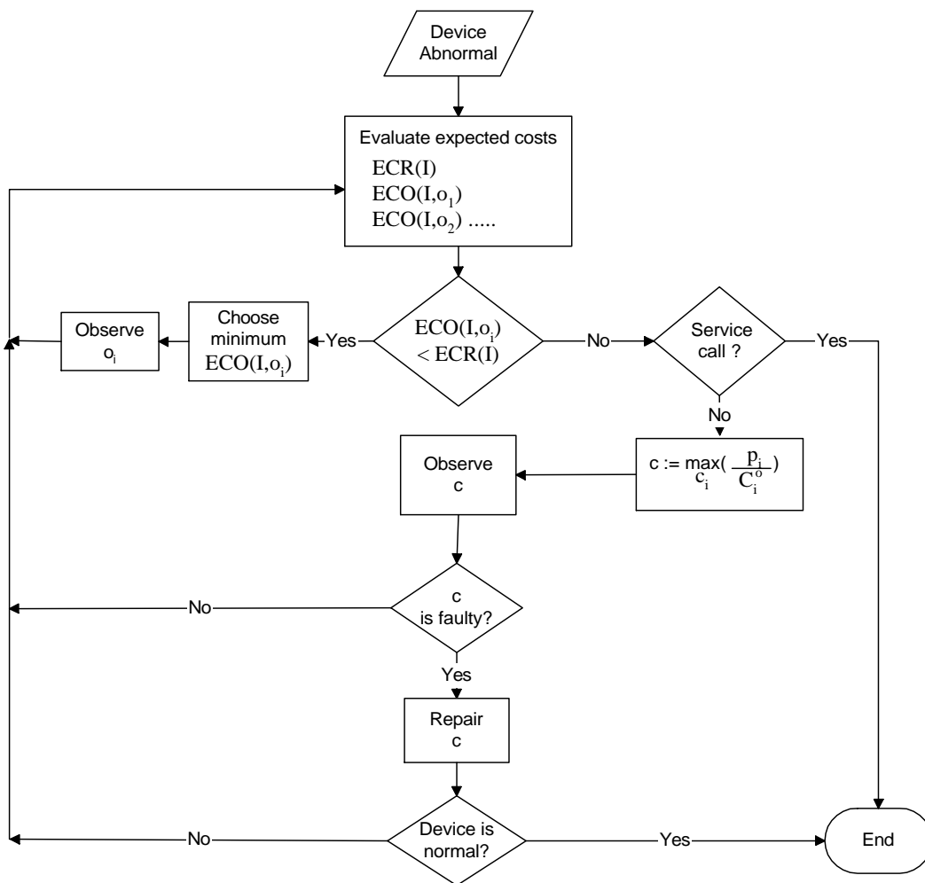
Figure 3: A summary of our approximate decision-theoretic method for generating a troubleshooting plan. First, we evaluate ECR(I) —the expected cost of repair under our current state of information I —and for every observation o_i , the expected cost of its observation ECO(I, o_i) . Next, if there is an observation o_i for which ECO(I, o_i) < ECR(I) , then we observe o_i for which ECO(I, o_i) is a minimum. Otherwise, we check to see whether or not we should call service. We do so if and only if n_s , given by Equation 2, is equal to zero. If so, then we call service and then quit. Otherwise, we perform an observation–repair action on the component c_i such that p_i/C_i^o is a maximum. If we repair c_i , then we check if the device is functioning properly. If it is, then we quit, otherwise we repeat the process, identifying the next best action.
