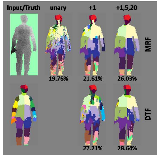
Figure 4. Body-parts recognition results (30 training images). MRF (top), DTF (bottom). Accuracy is shown below each result. Note the improvement in labeling of the shoulder and upper torso.
