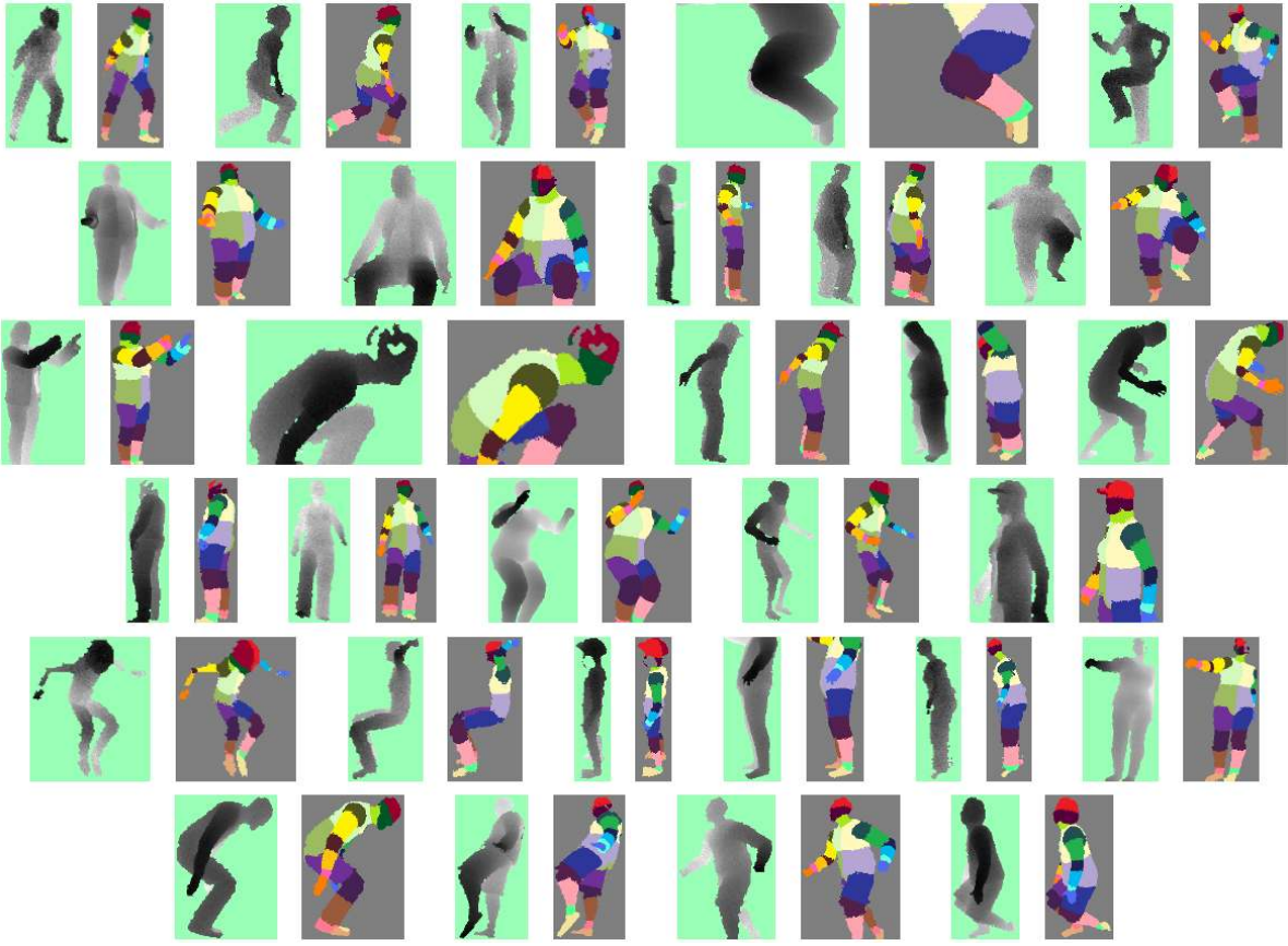
Figure 9. Train set used for body-part recognition. Depth map next to ground-truth labeling.
