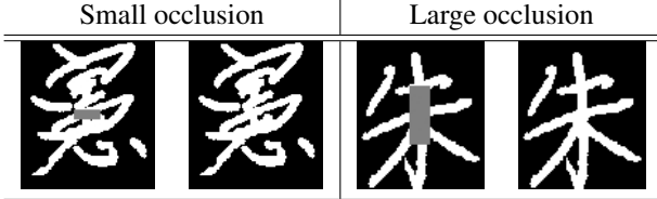
Figure 1. Completing small and large occluded boxes of Chinese characters: test (left) and ground truth (right).
