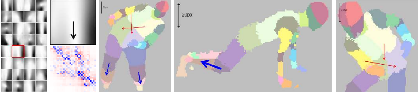
Figure 5. Illustrating one learned vertical interaction (20 pixels apart): The average depth-normalized silhouette reaching one of the 32 leaf nodes in the learned decision tree for the vertical pairwise interaction is shown on the left. Note how these patterns differ from those of Figure 10 in the main paper. For one specific leaf node (marked in red) the corresponding pattern and learned weight matrix is shown in the second column. The top two attractive terms (blue) and repulsive terms (red) are illustrated as arrows on poses taken from the test set (right). The first pose shows how the knee on top of the lower leg (both left and right) are plausible (vertical) configurations where the learned patch is matched. However, for the second pose the leaf pattern is not matched and indeed this (not-vertical) configuration is no longer valid. The first and third pose show that the left-arm-over-right-torso, and right-upper-torso-over-left-lower-torso are plausible (vertical) configurations, but only when the leaf pattern is not matched. Therefore these (vertical) configuration are inhibited for this specific leaf.
