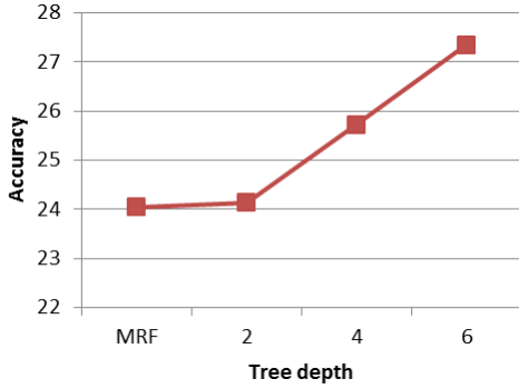
Figure 2. Body parts recognition results (30 training images): For neighborhood size +1,5,20 we increase the depth of the pair-wise trees from 1 (MRF) to 6, and record the resulting accuracy.
