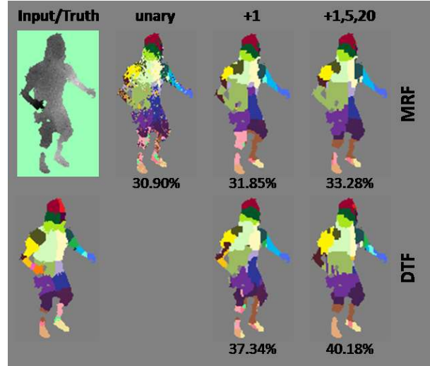
Figure 3. Body-parts recognition results (30 training images). MRF (top), DTF (bottom). Accuracy is shown below each result. Note the improvement in labeling the arm and elbow parts. (Notice that DTF unary is the same configuration as MRF unary).
