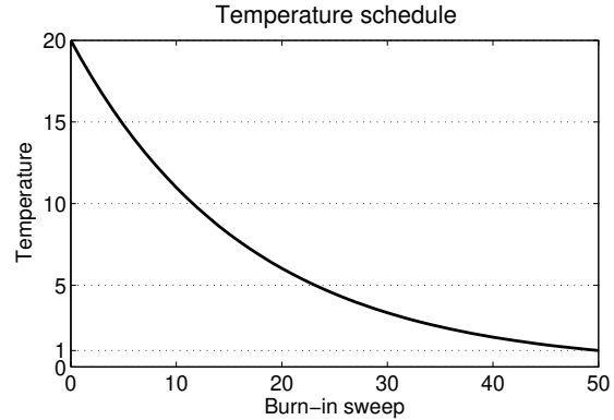
Figure 7. Temperature schedule used for the burn-in phase of the Gibbs sampler and during simulated annealing.
