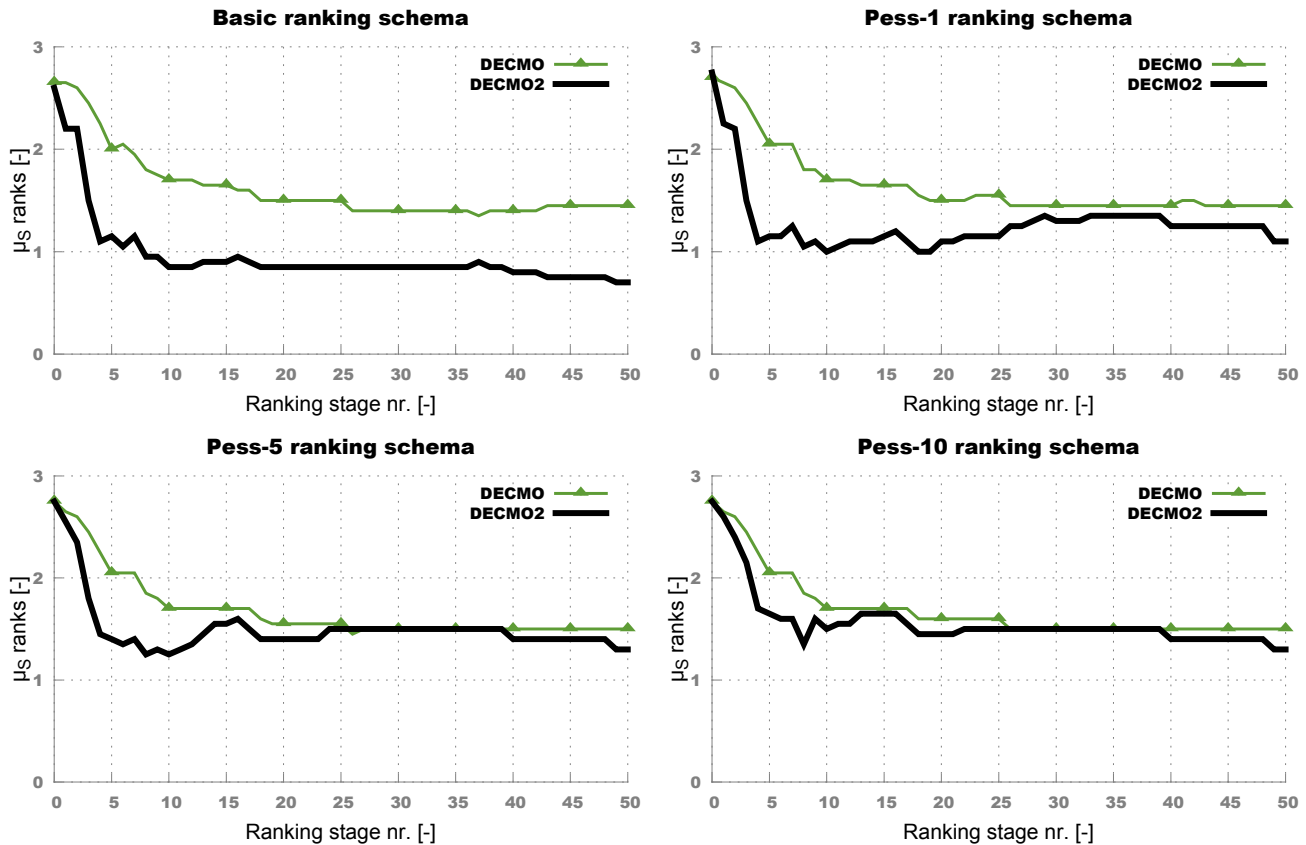
Fig. 8 HRPCs obtained when comparing DECMO2 with DECMO over 20 artificial benchmark MOOPs
