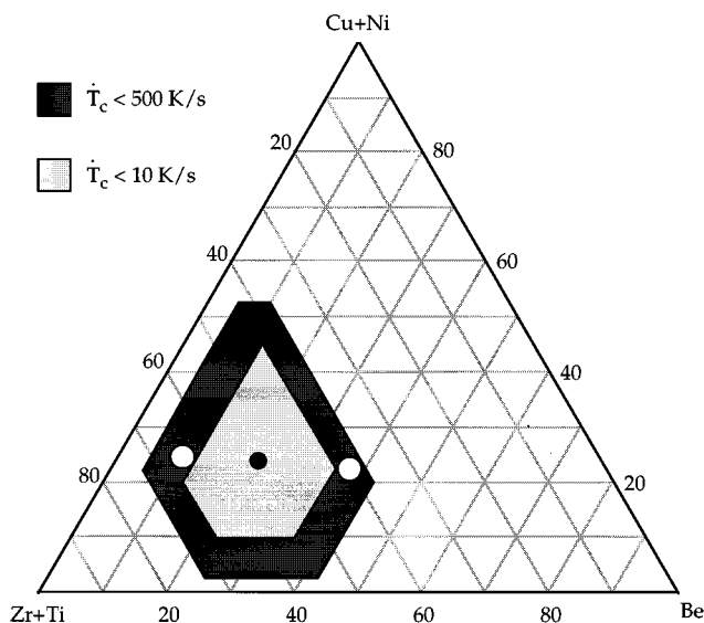
FIG. 4. Quasi-ternary cut through the (Zr–Ti)–(Cu–Ni)–Be phase diagram. The compositions of the initial Zr_{41.2}Ti_{13.8}Cu_{12.5}Ni_{10.0}Be_{22.5} melt (●) and the approximate compositions of the two resulting phases (○) are marked.
