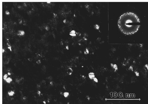
FIG. 3. Dark field TEM image of a Zr_{41.2}Ti_{13.8}Cu_{12.5}Ni_{10.0}Be_{22.5} alloy after primary crystallization.
