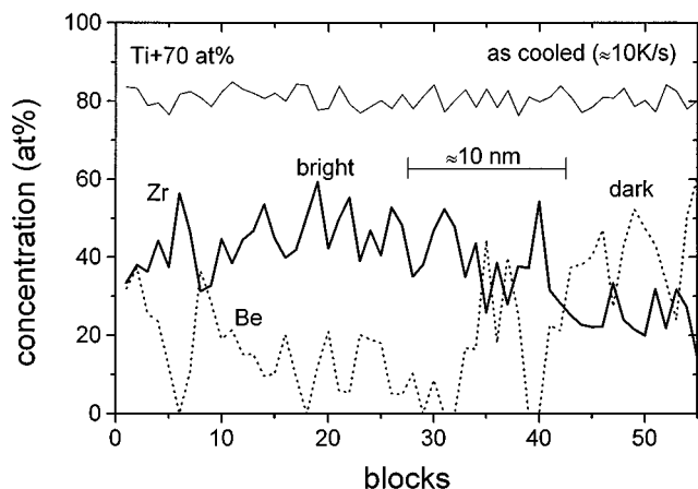
FIG. 2. Atom probe concentration profile from the center of an amorphous Zr_{41.2}Ti_{13.8}Cu_{12.5}Ni_{10.0}Be_{22.5} sample rod. The Zr-rich regions appear bright and the Be-rich regions appear dark on the FIM images.
