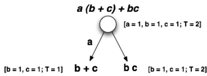
Fig. 7. Weight Assignment Example
