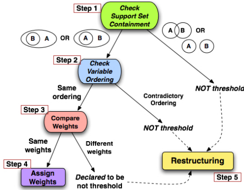
Fig. 4. The Threshold Decomposition Flow
