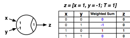
Fig. 1. Threshold gate example
