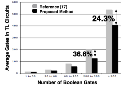
Fig. 11. Comparison of results
