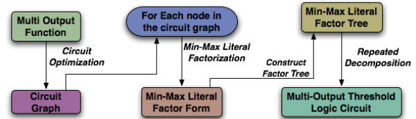
Fig. 10. The Threshold Synthesis Flow
