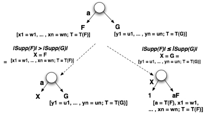
Fig. 8. Restructuring Rules
