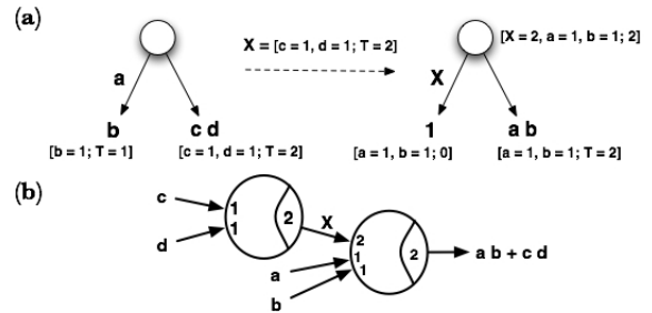
Fig. 9. Synthesis Example: (a) Synthesis procedure. (b) Synthesized circuit
