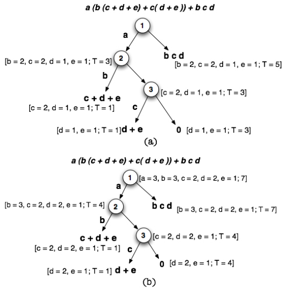
Fig. 6. Resynthesis Example
