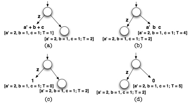
Fig. 5. Weight-threshold assignment to leaf nodes
