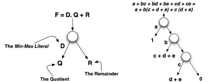
Fig. 2. The Min-Max Literal Factor Tree Fig. 3. Example Factor Tree
