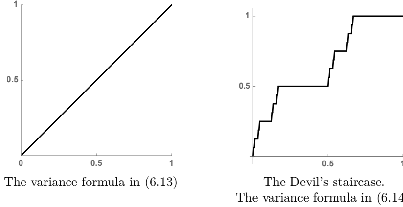
Fig. 8. The two cumulative distributions
