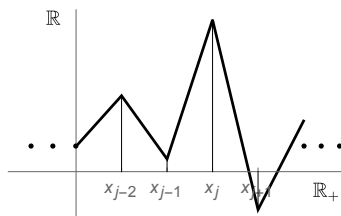
Fig. 13. Piecewise linear spline
