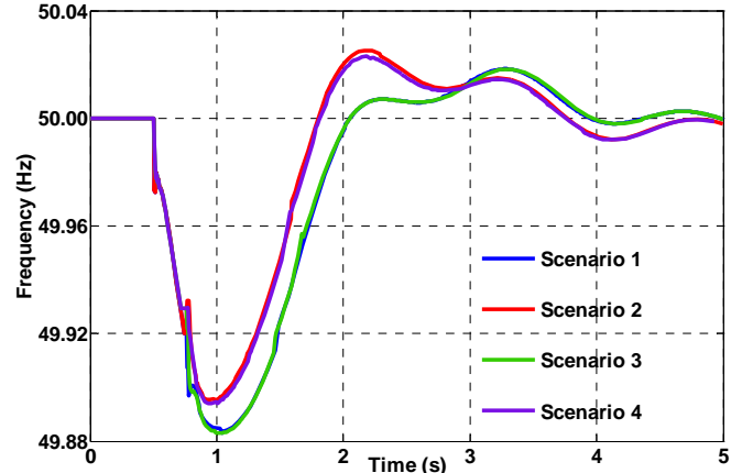
Fig. 17. Frequency variation with different scenarios.
