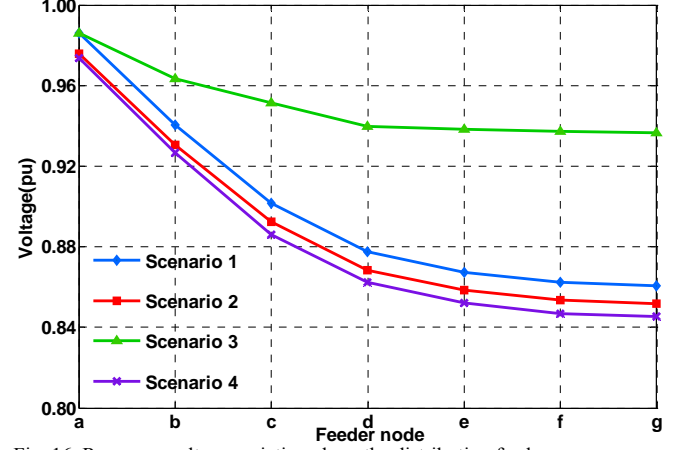
Fig. 16. Recovery voltage variation along the distribution feeder.
