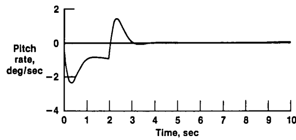
(a) Pitch rate.
