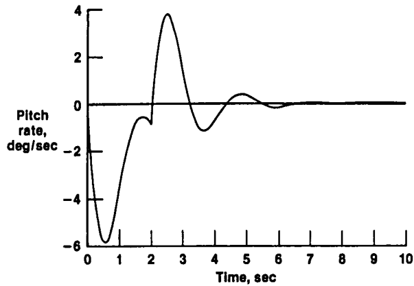
(a) Pitch rate.
