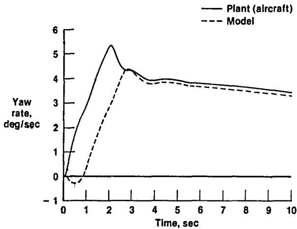
(a) Yaw rate.
