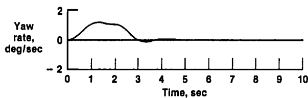
(b) Yaw rate.
