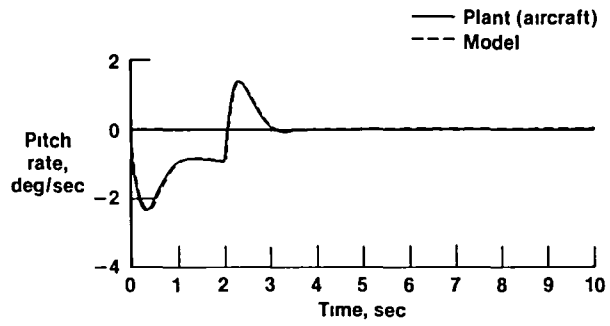
Fig. 4 Model-following response to elevator command input.
