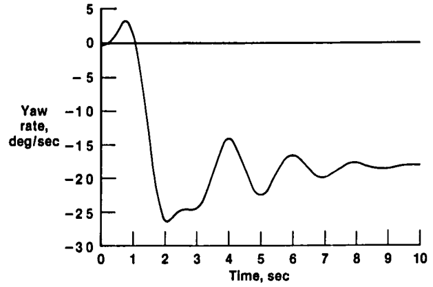
(b) Yaw rate.
