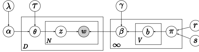
Figure 1: A graphical model representation for sparseTMs.
