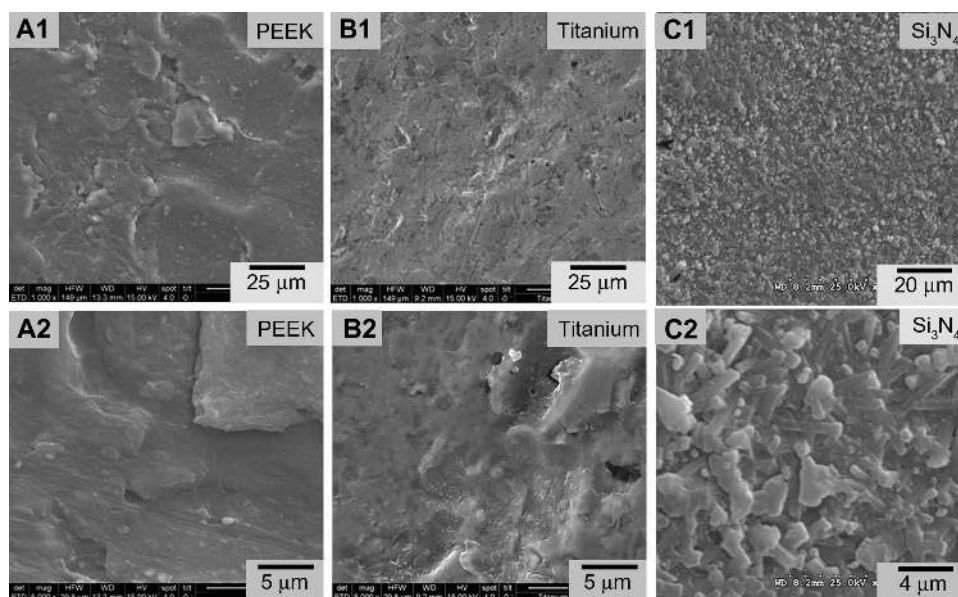
Figure 1 Scanning electron microscopy surface microstructures of PEEK Optima®, Ti, and \text{Si}_3\text{N}_4 ; (A1) PEEK 1000 \times ; (A2) PEEK 5000 \times ; (B1) Ti 1000 \times ; (B2) Ti 5000 \times ; (C1) \text{Si}_3\text{N}_4 1000 \times ; (C2) \text{Si}_3\text{N}_4 5000 \times .
