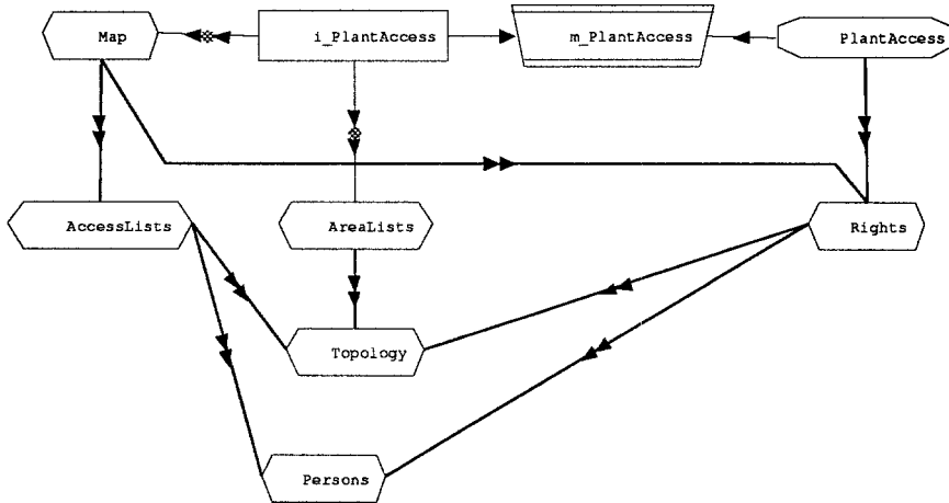
Fig. 2. A Development Graph
