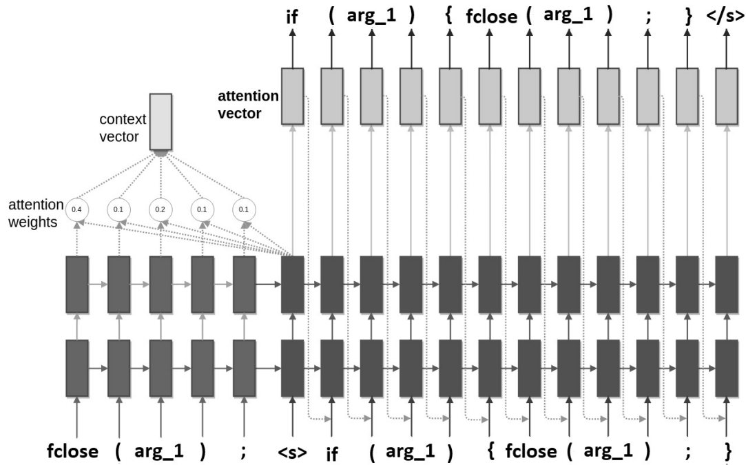
Fig. 3. Example of a deep recurrent architecture for transforming
