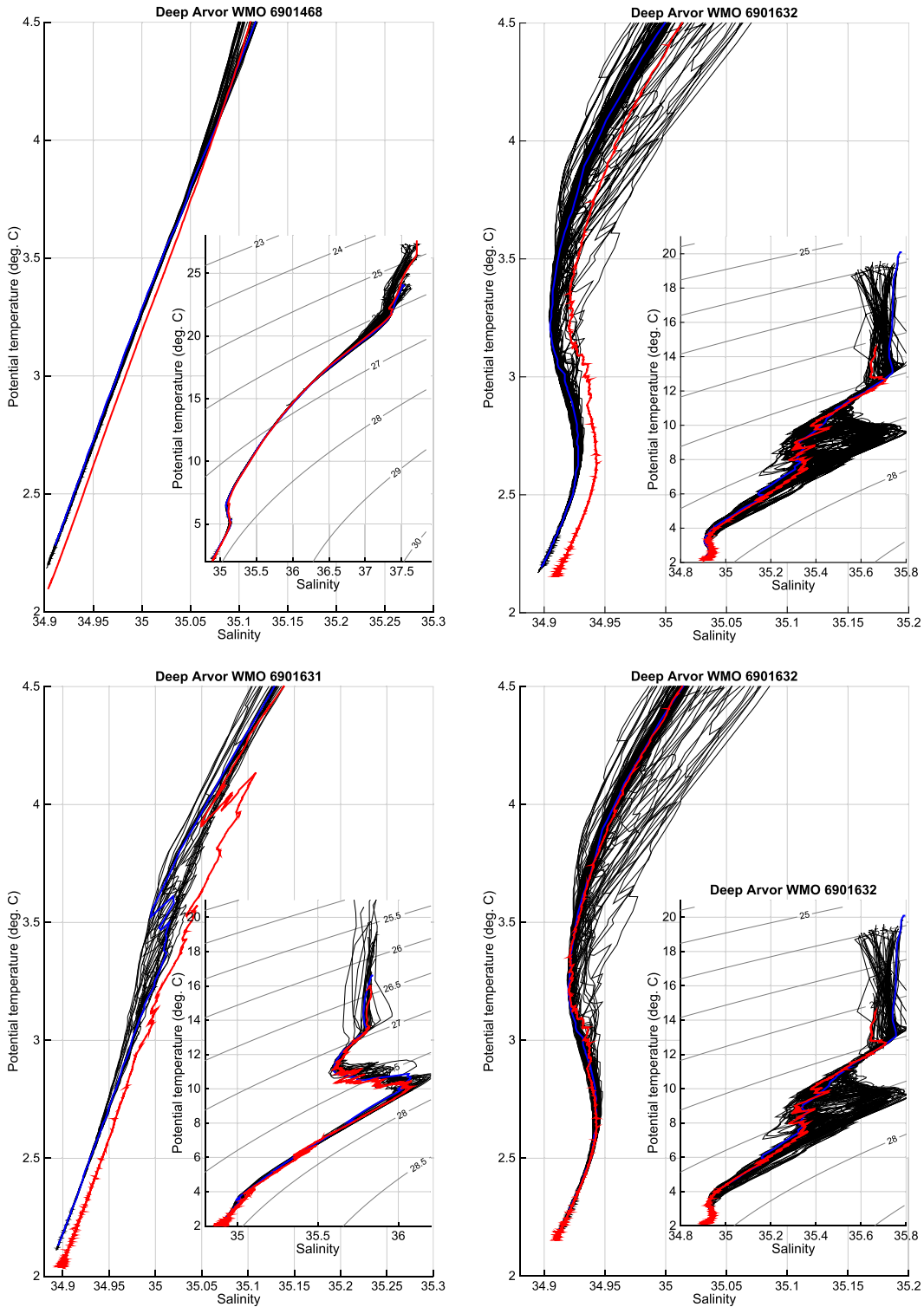
FIG. 15. A \theta/S diagram for the Deep-Arvor floats (upper left) 6901468, (lower left) 6901631, (upper right) 6901632, and (lower right) 6901632 in using the corrected salinity following the OW method. In each panel, the large figure is the \theta/S diagram in the deep layers, while the \theta/S diagram in the inset represents the diagram for the full water column. Deep-Arvor floats data (black curves). Calibrated reference profiles collected at float deployment (red curves). Nearest float profile compared to the calibrated reference profile (blue curves).
