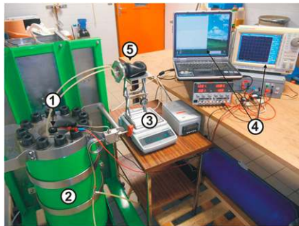
FIG. 6. (left) Hydraulic test bench used for the assessment of the pump efficiency. Hydraulic end cap under test (1). Hyperbaric test tank (2). Scales to weigh the oil transfers during pump or valve activations (3). Computers and oscilloscope for monitoring and control (4). Oil reservoir (5). (right) Current absorbed by the pump during oil transfers.
