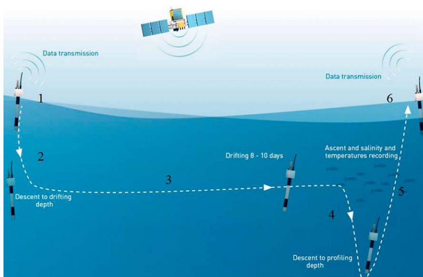
FIG. 1. Typical operational cycle of an Argo profiling float (courtesy of Euro-Argo Research Infrastructure). The float reduces its buoyancy (1), dives (2), and drifts at parking depth (3). Then it travels to the profile depth (4) and makes its measurement during the ascent (5). Transmissions and positioning are done at surface at the end of each cycle (6).
