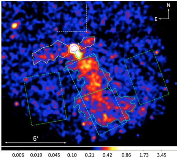
Figure 2. Merged 0.5–8 keV exposure-corrected image produced from all 8 ACIS-I observations with point sources (detected by wavdetect ) removed. The image is binned by a factor of 8 ( 3''.9 pixel size), and smoothed with an r = 11''.8 Gaussian kernel. The following spectral extraction regions are shown: the tail (green contour region; the line separates the “near” and “far” halves), and the “whiskers” (yellow polygons on either side of the CN). The two green dashed rectangles to the sides of the tail are the background regions used in the tail’s spectral fits. The cyan 2'.5 \times 6'.2 rectangular region (along the tail contour) is used to extract the tail brightness profile (see Figure 5). The CN (magenta polygon) and stem (green polygon) are also shown (same regions as in Figure 2), along with the background region (dashed white box) used in the pulsar, CN, stem, and whiskers spectral fits. The level for the green contour was chosen in such a way that it conforms to the tail morphology at the contrast shown. The color bar is in units of counts \text{arcsec}^{-2} .
