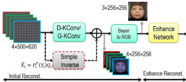
Figure 4. Our FlatCam reconstruction network with and without (including dashed-line block) residual learning.
