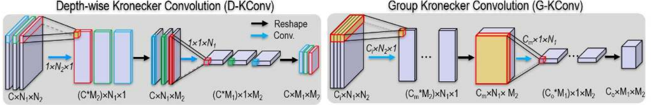
Figure 2. Depth-wise (D-KConv) and Group Kronecker convolution (G-KConv). G-KConv utilizes information across channels with more flexible parameters ( C_m and C_o represent the numbers of intermediate and output features, respectively) than D-KConv.
