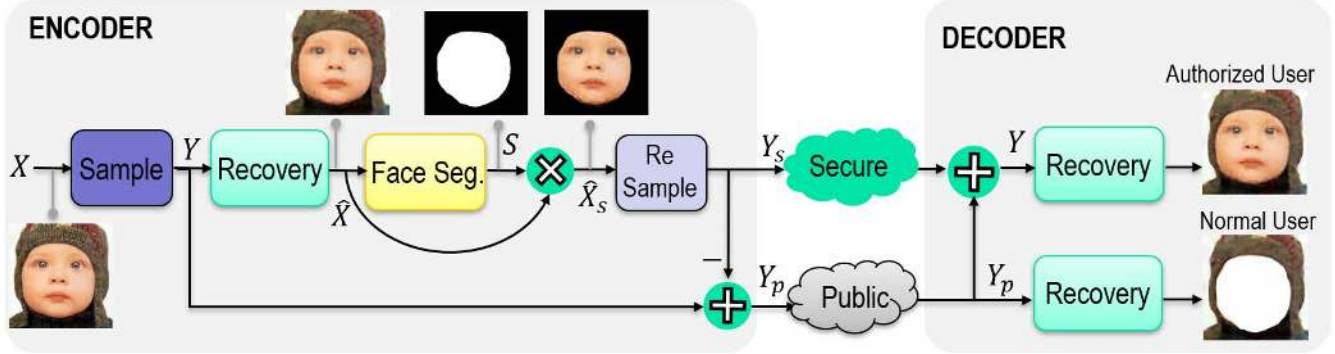
Figure 3. Our deep visual privacy protection network. The facial region in reconstructed image of normal user is protected (it was converted to white for better visualization).
