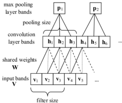
Fig. 1. Diagram showing a typical convolutional network architecture consisting of a convolutional and max-pooling layer. In this diagram, weights with the same line style are shared across all convolutional layer bands. Note this figure shows non-overlapping pooling, which is different than [10].
