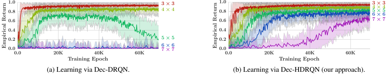
Figure 2. Task specialization for MAMT domain with n = 2 agents, P_f = 0.3 . (a) Without hysteresis Dec-DRQN policies destabilize in the 5 \times 5 task and fails to learn in the 6 \times 6 and 7 \times 7 tasks. (b) Dec-HDRQN (our approach) performs well in all tasks.
