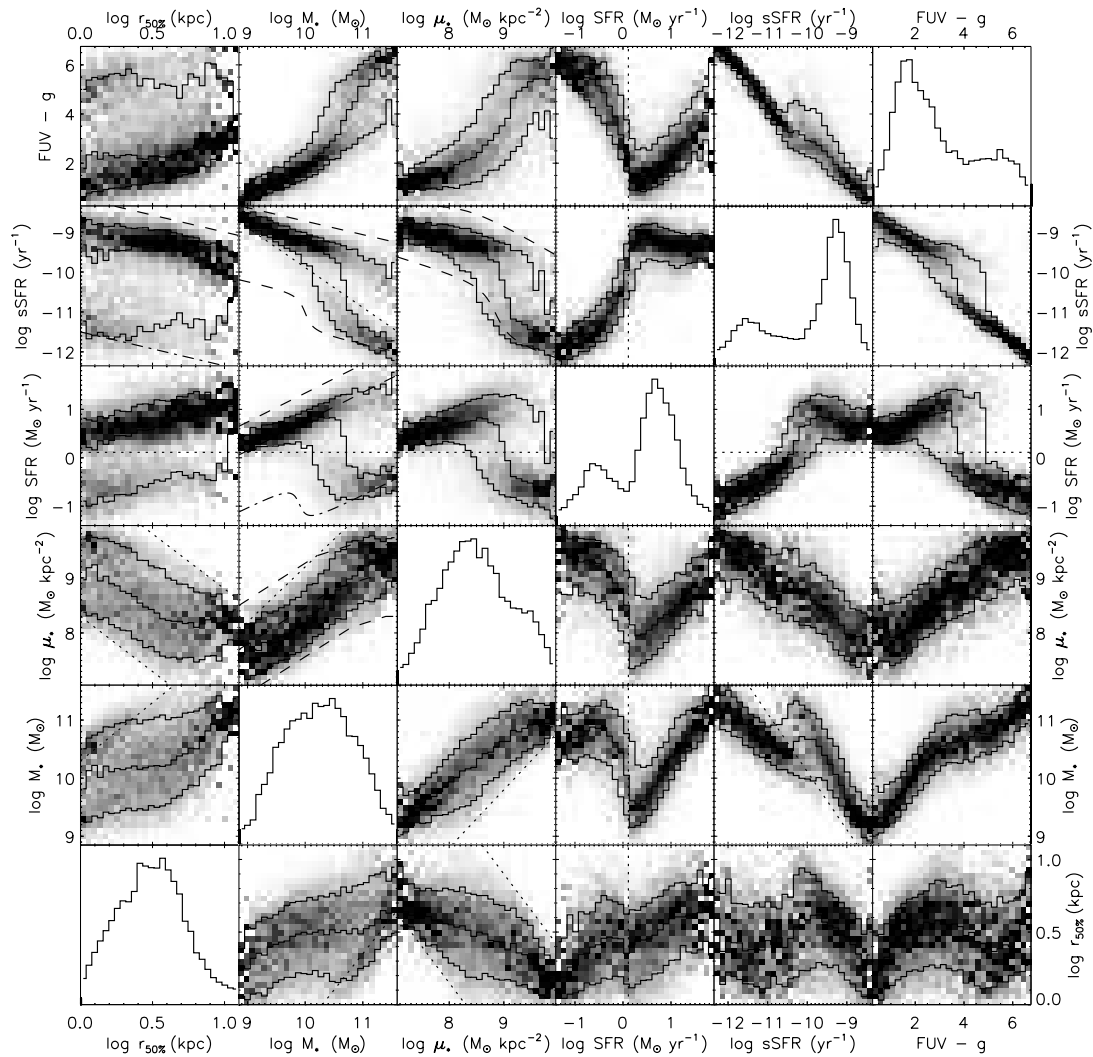
Fig. 8.—Conditional plot of Fig. 7, that is, with each column being normalized separately. The solid lines represent the 10%, 50%, and 90% quantiles in every column. We reiterate that star formation rates below our UV-detection limit have been obtained through SED extrapolation and are prone to large uncertainties.
