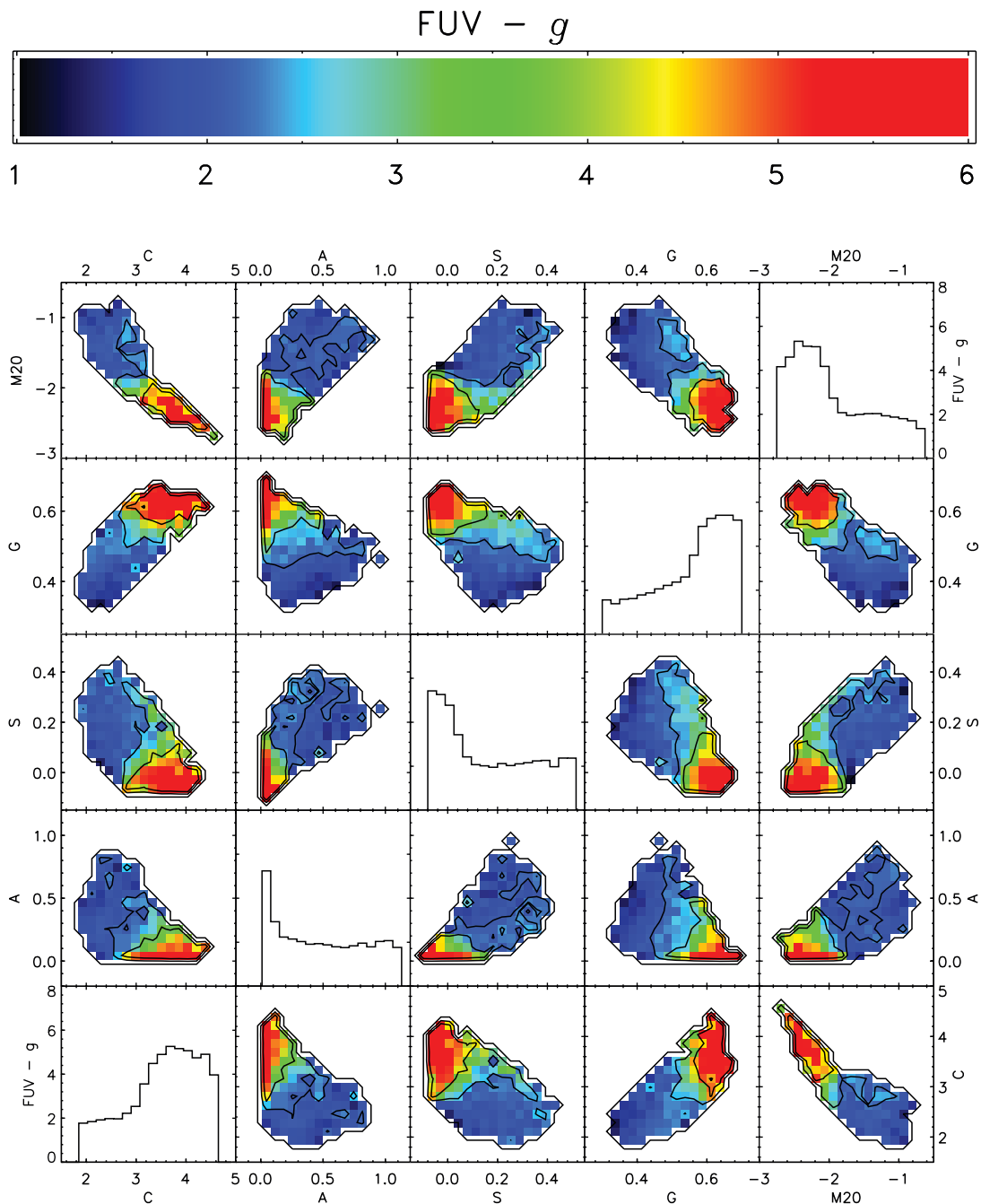
FIG. 17.—Rest-frame FUV- g color as a function of each as well as of each combination of two morphological parameters for our full sample. The value in each color bin as well as in each histogram bin was obtained by taking the median FUV- g color of all the objects present in that bin. Bins with fewer than 10 objects were removed. The color scale for histograms is indicated by the thin font topmost y -axis on the right side of the figure as well as the bottom-most y -axis on the left side of the figure.
