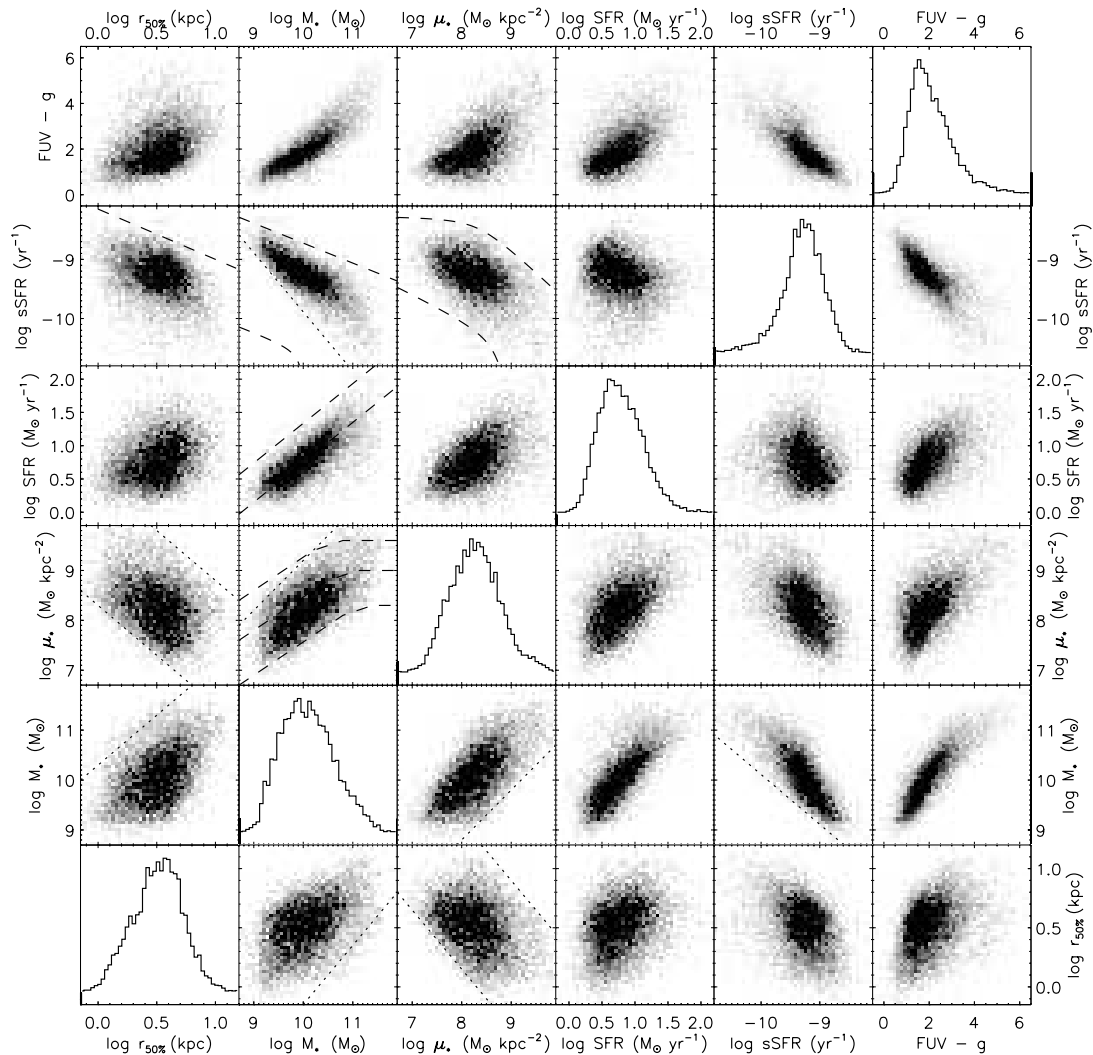
Fig. 6.—Distribution of our UV-detected sample in various physical parameters. Dotted lines represent: in the \log M_* – \log sSFR plane, our detection limit of \log SFR = 0.11; in the \log \mu_* – \log r_{50\%} plane, our detection limit of \log M_* = 9.1 and the line of \log M_* = 11.6 (which is the high-mass cutoff in our mass distribution); in the \log \mu_* – \log M_* plane, our detection limit of r_{50\%} = 1.0 kpc; in the \log M_* – \log r_{50\%} plane, the line of \log \mu_* = 9.5 (which represents the typical value for ellipticals). Dashed lines represent, in the \log sSFR vs. \log r_{50\%} plane, the upper envelope of the Brinchmann et al. (2004) local relation shifted up by 0.45; in \log sSFR vs. \log M_* , the upper and lower envelopes of the Brinchmann et al. (2004) local relation shifted up by 0.55; in \log sSFR vs. \log \mu_* , the upper and lower envelopes of the Brinchmann et al. (2004) local relation shifted up by 0.45; in \log SFR vs. \log M_* , the median for blue galaxies as well as the upper envelope of the local relation of Brinchmann et al. (2004) obtained from their raw fiber measurements (their Fig. 17), both shifted up by 0.35; and in \log \mu_* vs. \log M_* , the upper and lower envelopes as well as the median of the local relation from Kauffmann et al. (2003b) (unadjusted).
