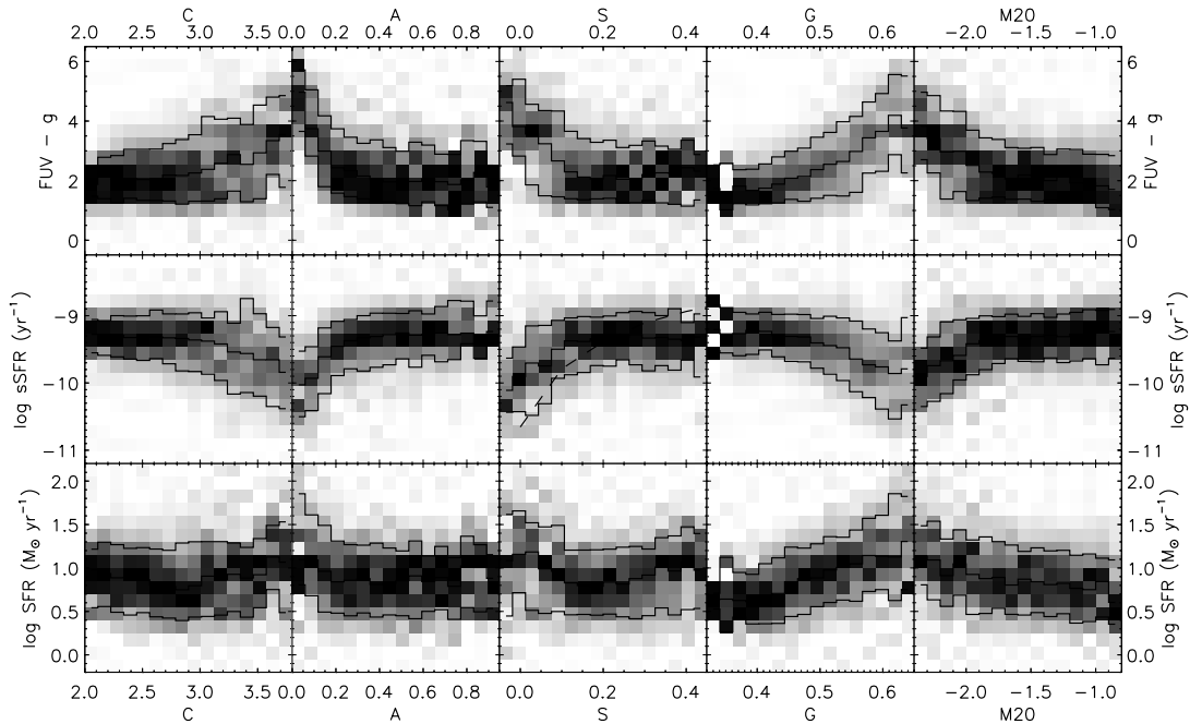
FIG. 16.— Conditional plot (i.e., with each column separately normalized) of color, absolute and specific star formation rates of our UV-detected and size-complete sample as a function of morphological parameters. The solid lines represent the 10%, 50%, and 90% quantiles in every column. The dashed line in sSFR vs. S represent the relation of Conselice (2003) normalized to z = 0.7 and to our distribution in S .
