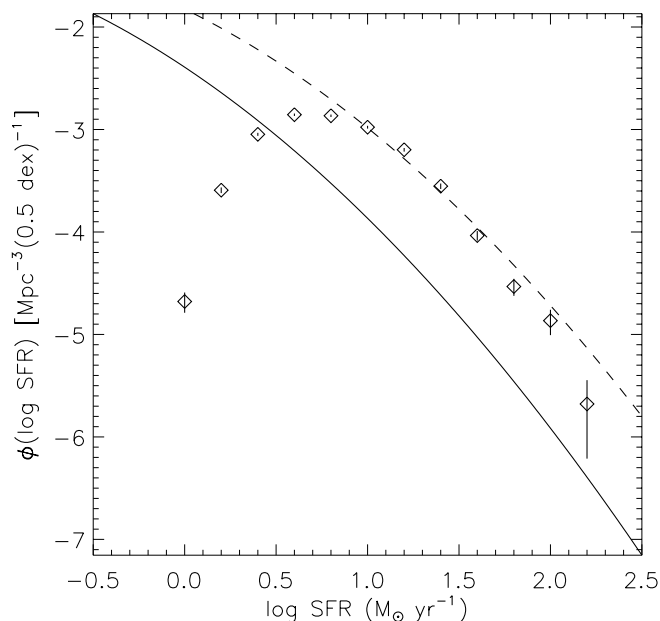
Fig. 9.—Star formation rate distribution in our UV-detected sample compared to the local star formation rate function of Martin et al. (2005b) ( solid line ) and to the same function shift by 0.55 in log SFR ( dashed line ).
