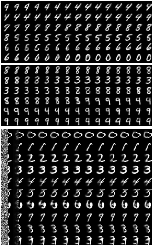
Figure 3. Top: two runs of consecutive samples (one row after the other) generated from 2-layer GSN model, showing fast mixing between classes, nice and sharp images. Note: only every fourth sample is shown; see the supplemental material for the samples in between. Bottom: conditional Markov chain, with the right half of the image clamped to one of the MNIST digit images and the left half successively resampled, illustrating the power of the generative model to stochastically fill-in missing inputs.
